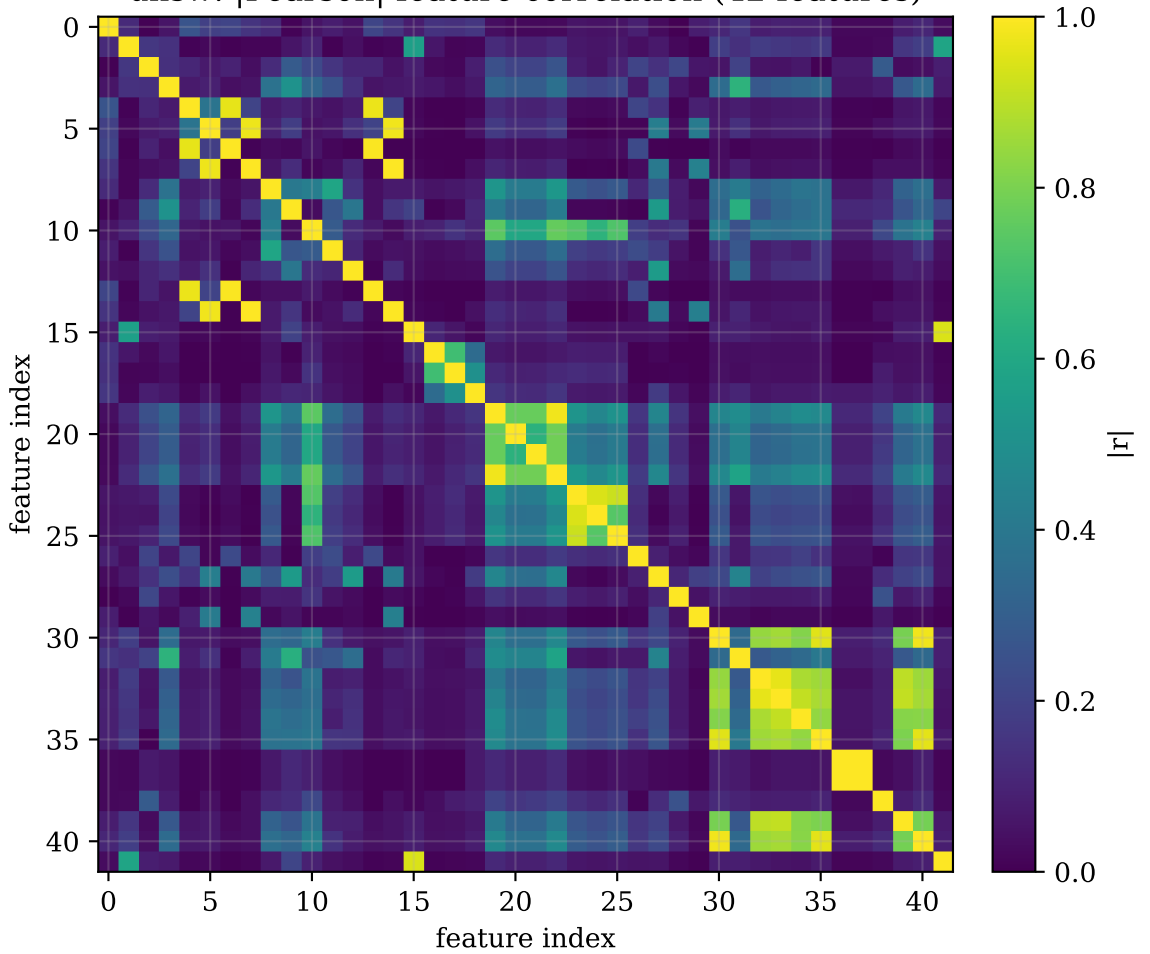
unsw: |Pearson| feature correlation (42 features)
