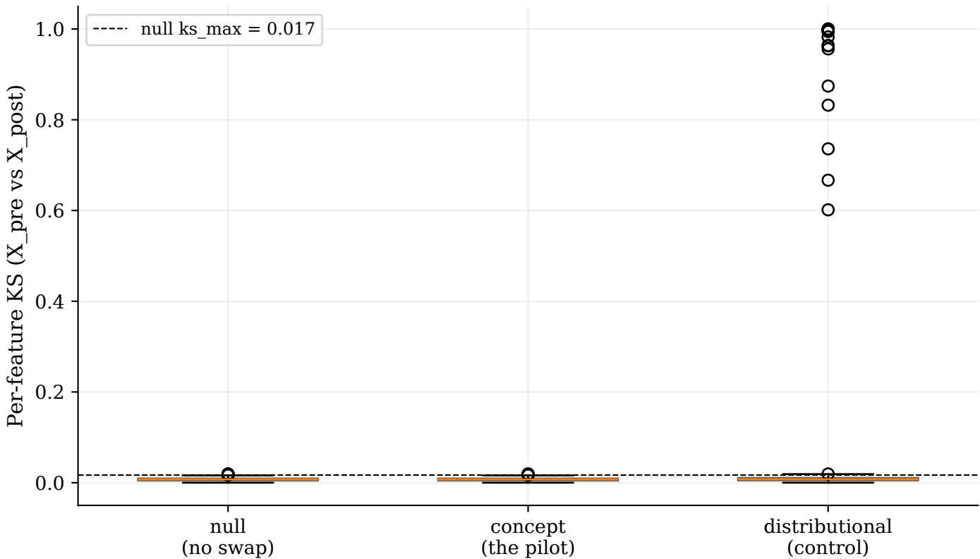
P(X) movement by arm: concept overlaps the sampling null
