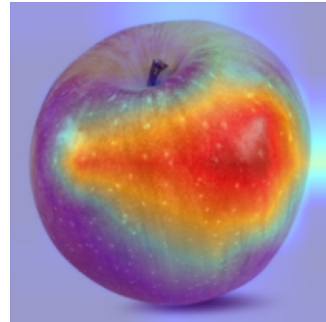
ResNet50
