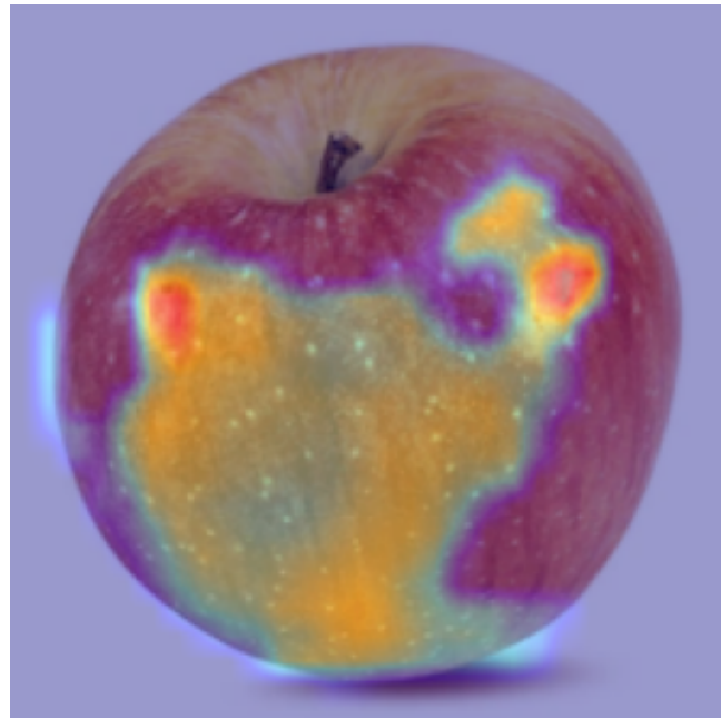
Custom CNN
