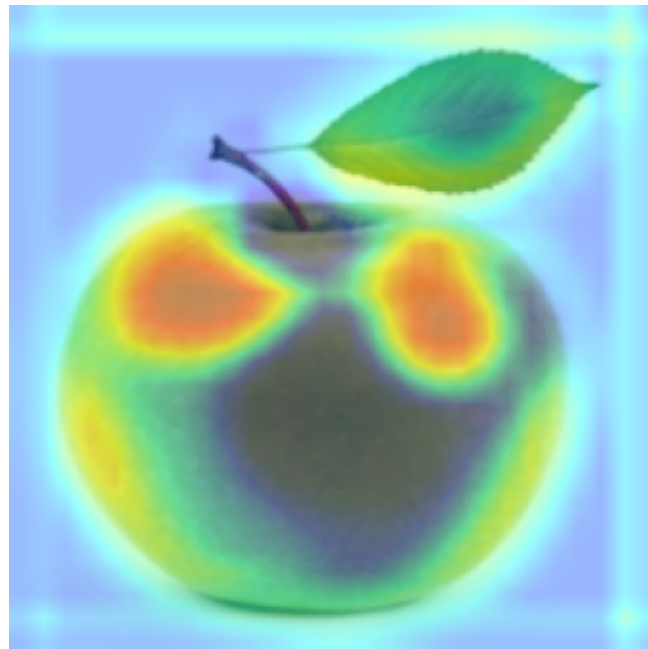
Custom CNN
