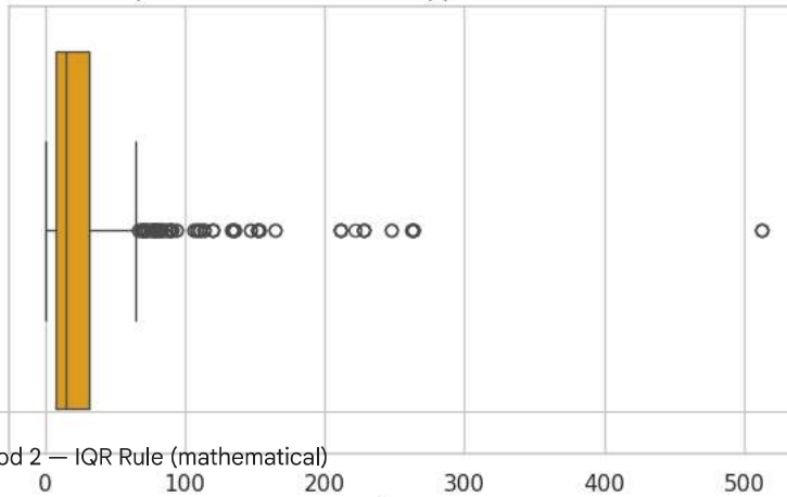
Boxplot of Fare — Outliers appear as individual dots
