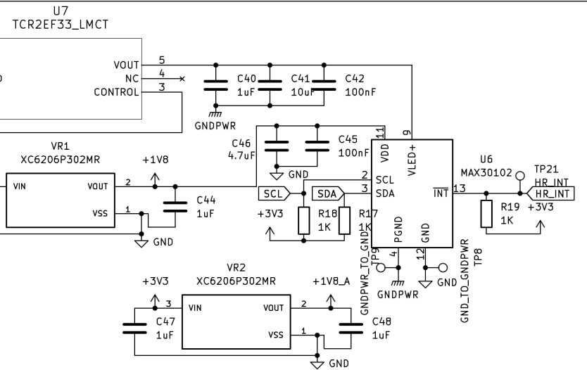
MAX30102 Heart Rate and Pulse Oximeter Circuit
