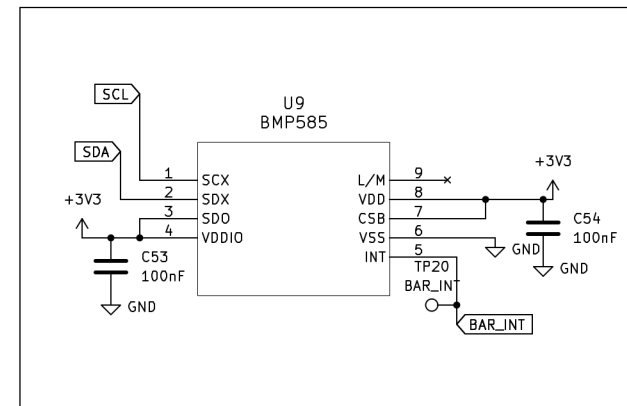
BMP585 Barometric Pressure Sensor Circuit
