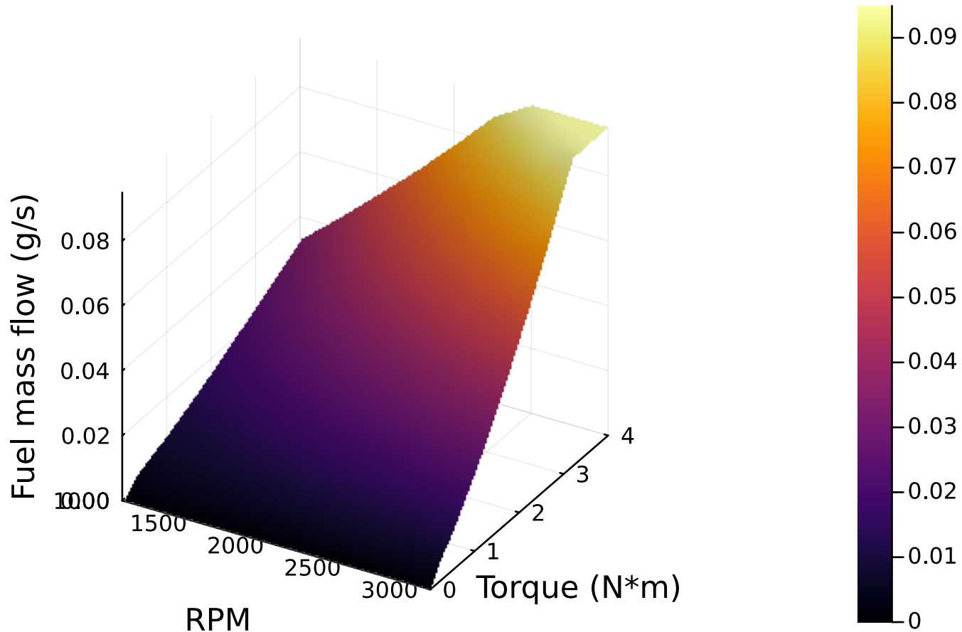
Diesel fuel flow map
