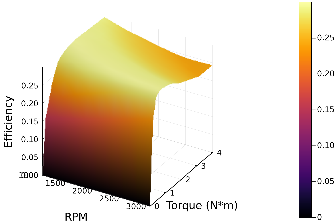
Diesel efficiency map
