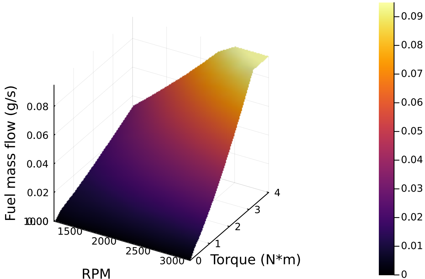
Diesel fuel flow map
