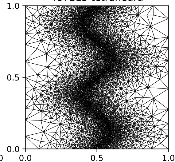
487213 tetrahedra
