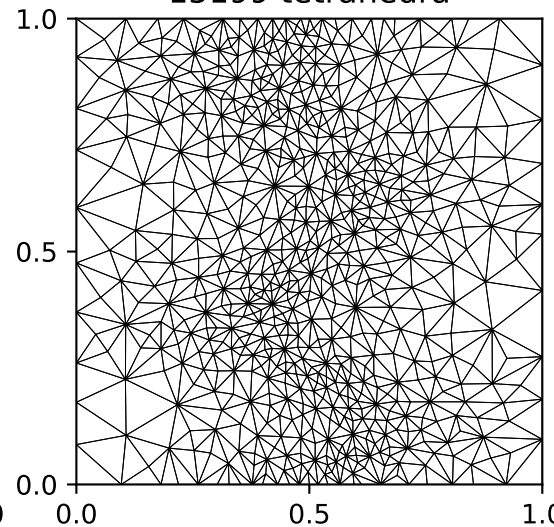
15199 tetrahedra
