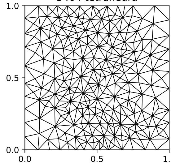
3404 tetrahedra
