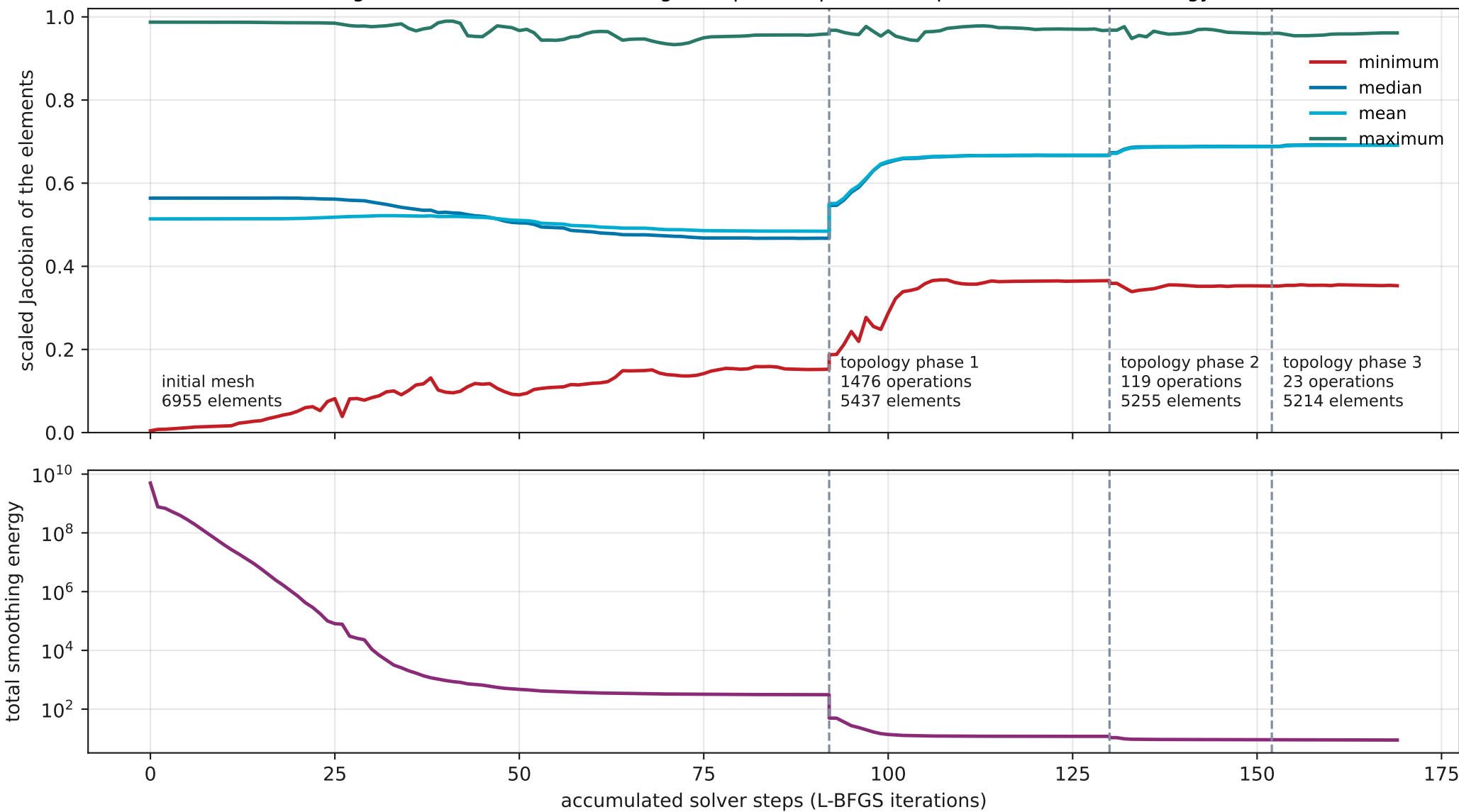
Distorted cube: smoothing (L-BFGS) alternated with edge swaps, collapses, and splits that lower the energy
