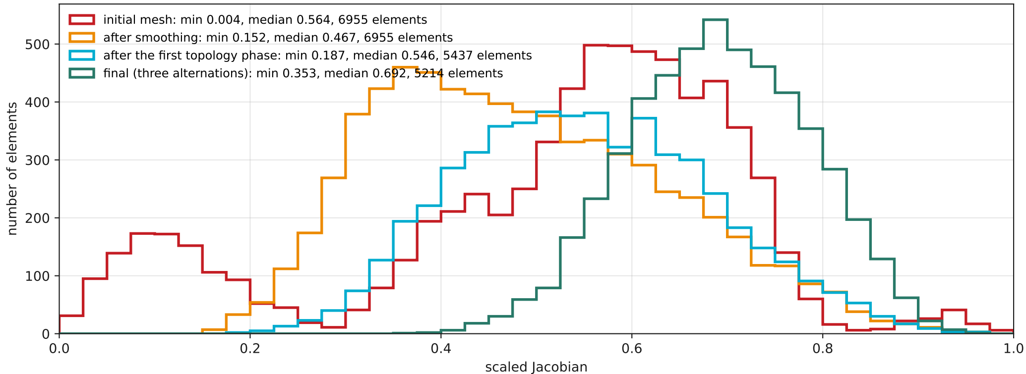
Distorted cube: distribution of the scaled Jacobian at four stages of the process
