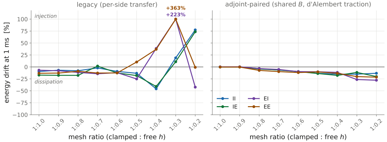
Figure 1: Non-overlap impedance Schwarz, energy drift at 1 ms across the mesh-ratio family, all four integrator combinations. Left: legacy per-side transfer (consistent-mass integer-step metric) — sign-indefinite, with injection up to +363% (EE) and +223% (EI) at 1:0.3. Right: the adjoint-paired coupling (staggered lumped-mass metric of Eq. (6) for explicit members) — monotone, sign-definite trace-jump dissipation at every ratio, and conservation to \leq 0.3\% on conforming and 1:0.9 meshes.
