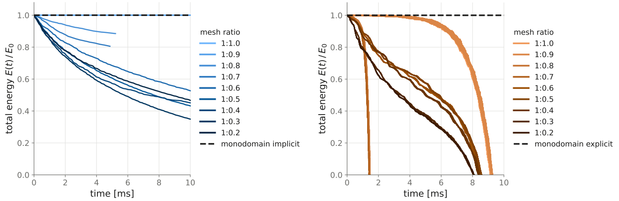
Figure 3: Adjoint-paired nonoverlap impedance Schwarz, 10 ms horizon, staggered energy metric. Left: implicit-implicit — no injection anywhere; conforming and 1:0.9 hold the monodomain reference, strong contrast dissipates monotonically, and the non-nested ratios 1:0.7–1:0.8 end early at \approx 5 ms (interface element inversion). Right: explicit-explicit — the staggered kinetic term goes secularly negative at every ratio as undamped grid-frequency content accumulates at \text{CFL} = 1 ; the 1:0.7–1:0.8 runs die of central-difference instability at 2.6–2.8 ms.
