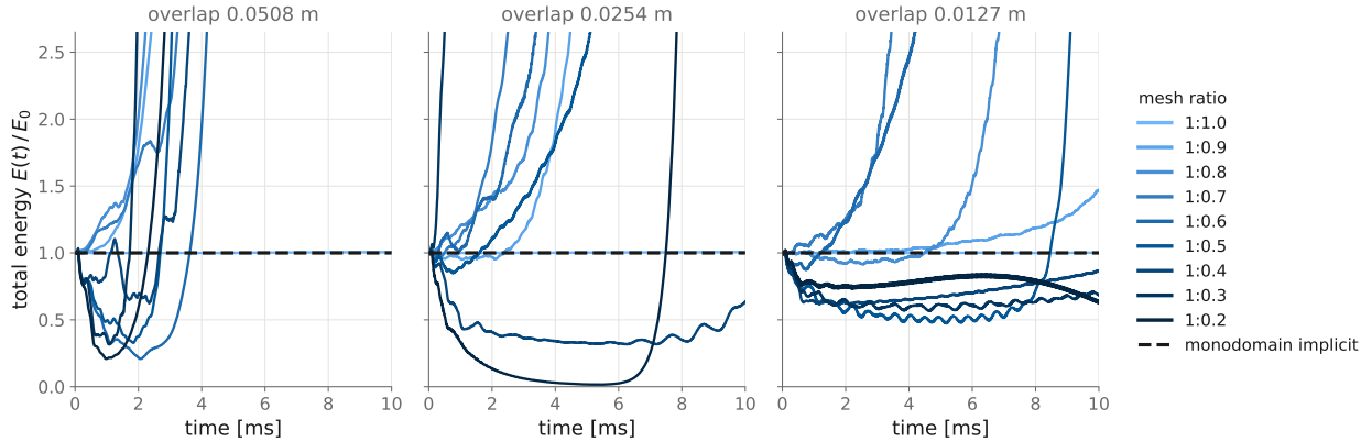
Figure 2: Overlap impedance Schwarz (variational transfer), implicit-implicit, 10 ms horizon. Nearly every nonconforming configuration either grows exponentially until element inversion kills the run (curves leaving the top of the axes) or collapses toward zero energy; only the conforming (1:1.0) runs track the monodomain reference. The mixed and all-explicit combinations (not shown) are worse: they lose even the conforming cases.
