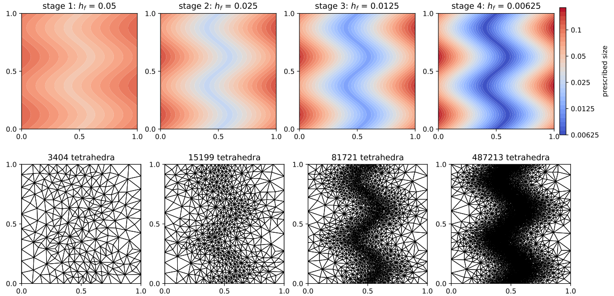
Figure 3: Plate refined toward a sinusoid: the prescribed size field and the top face of the mesh after each of the four stages.
