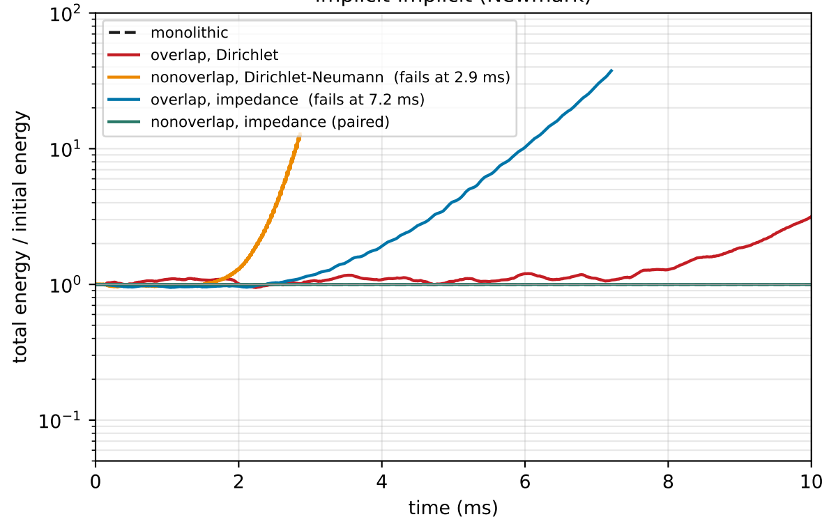
implicit-implicit (Newmark)
