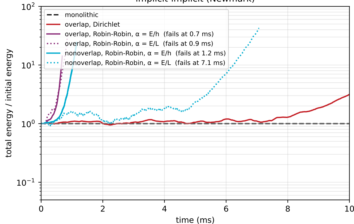
implicit-implicit (Newmark)
