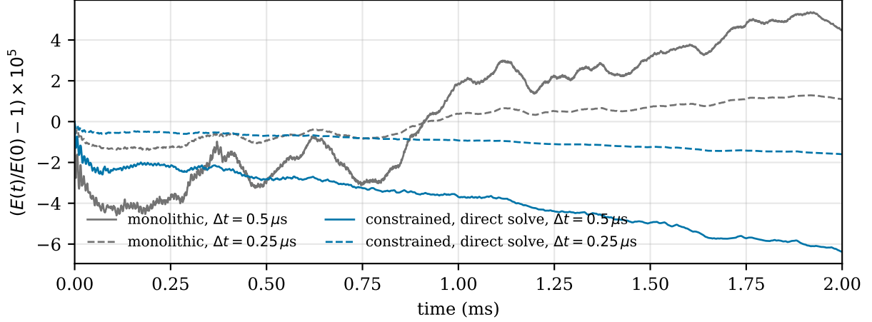
Figure 3: Energy of the neohookean cylinders, -35 m/s, 2 ms: the monolithic mesh and the decomposed mesh with the constrained exchange and the direct interface solve, each at two time steps.
