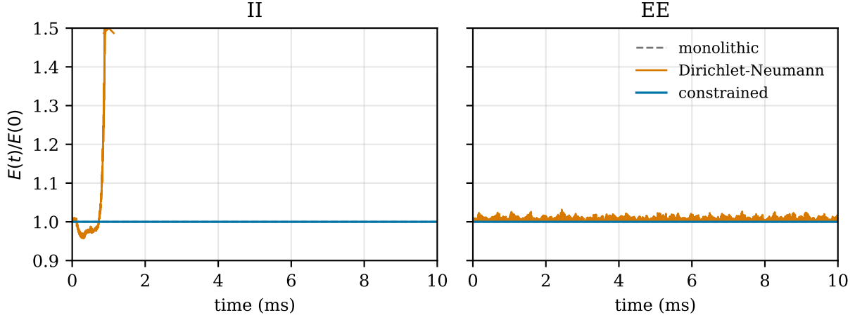
Figure 1: Energy of the conforming beam, stops of 1\mu s , 10 ms: the monolithic reference, the classical Dirichlet–Neumann exchange (Schwarz tolerance 10^{-8} on the displacement update, recursive Aitken), and the constrained exchange (tolerance 10^{-12} , Anderson acceleration). The classical exchange inverts an element at 1.0ms with implicit subdomains (cross); the constrained exchange coincides with the reference.
