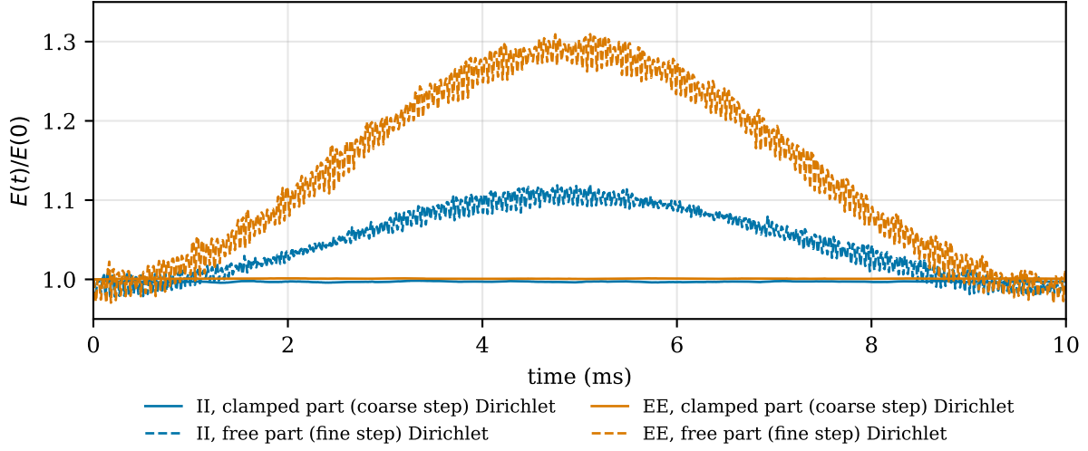
Figure 2: Energy of the conforming beam with the free part subcycled 4:1, tolerance 10^{-12} , Anderson acceleration. With the clamped part (coarse step) as the Dirichlet side the energy stays within 0.4%; with the free part (fine step) as the Dirichlet side it rises by 12% (II) and 31% (EE) and returns over the first bending period, while \tilde{E} stays constant to 10^{-9} in both arrangements.
