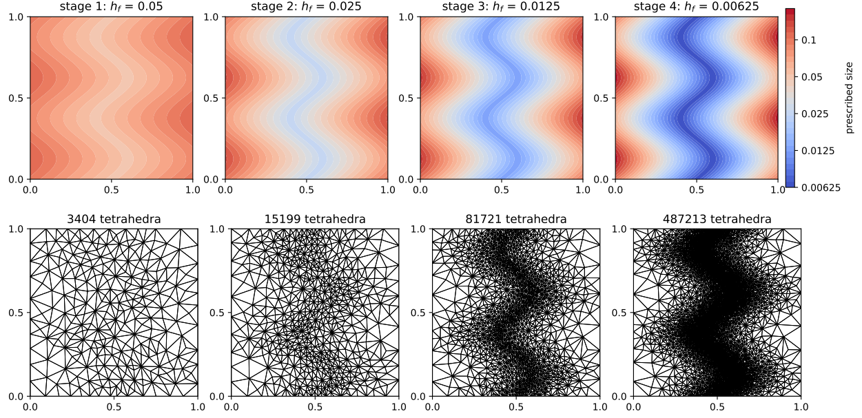
Figure 3: Plate refined toward a sinusoid: the prescribed size field and the top face of the mesh after each of the four stages.
