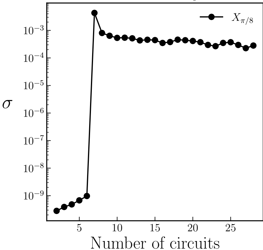
Gate Set Error vs. Sample Size
