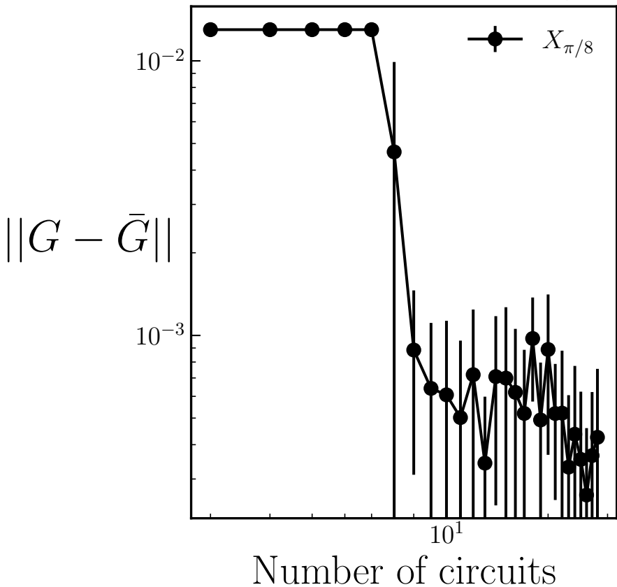
Gate Estimation Error vs. Number of Circuits, N = 5
