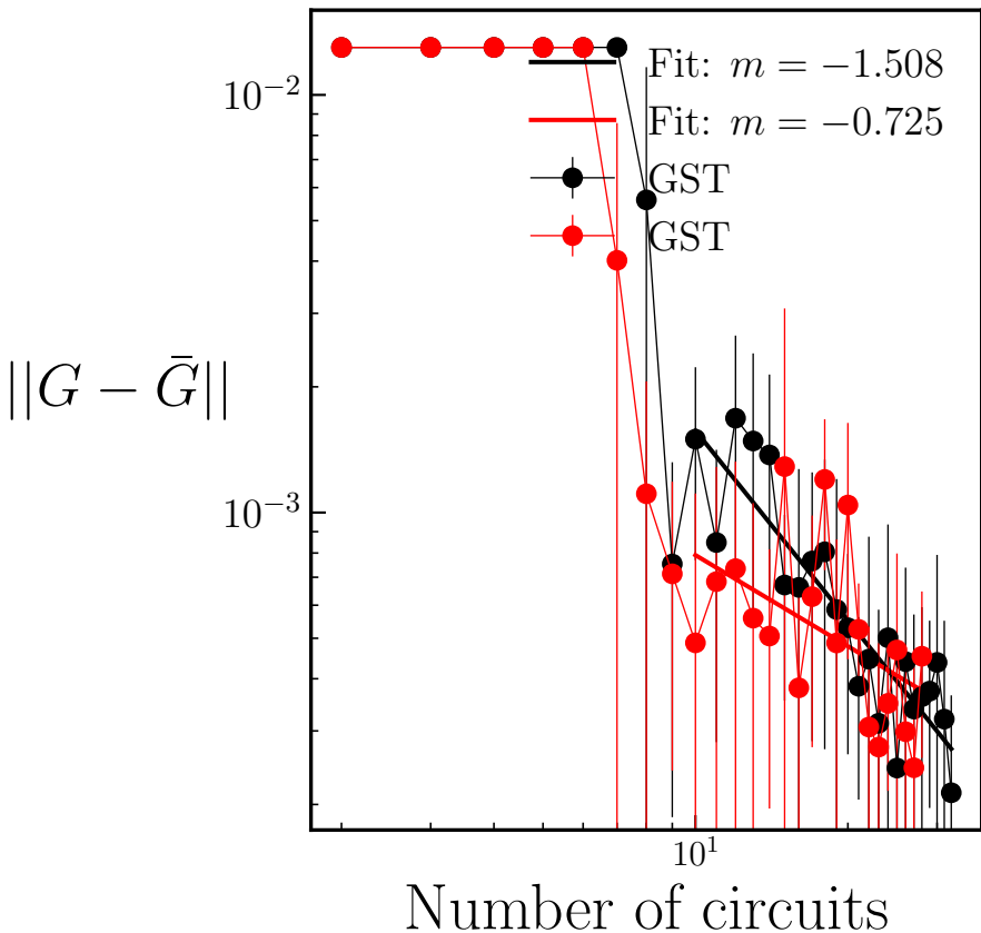
Gate Set Error vs. N circuits
