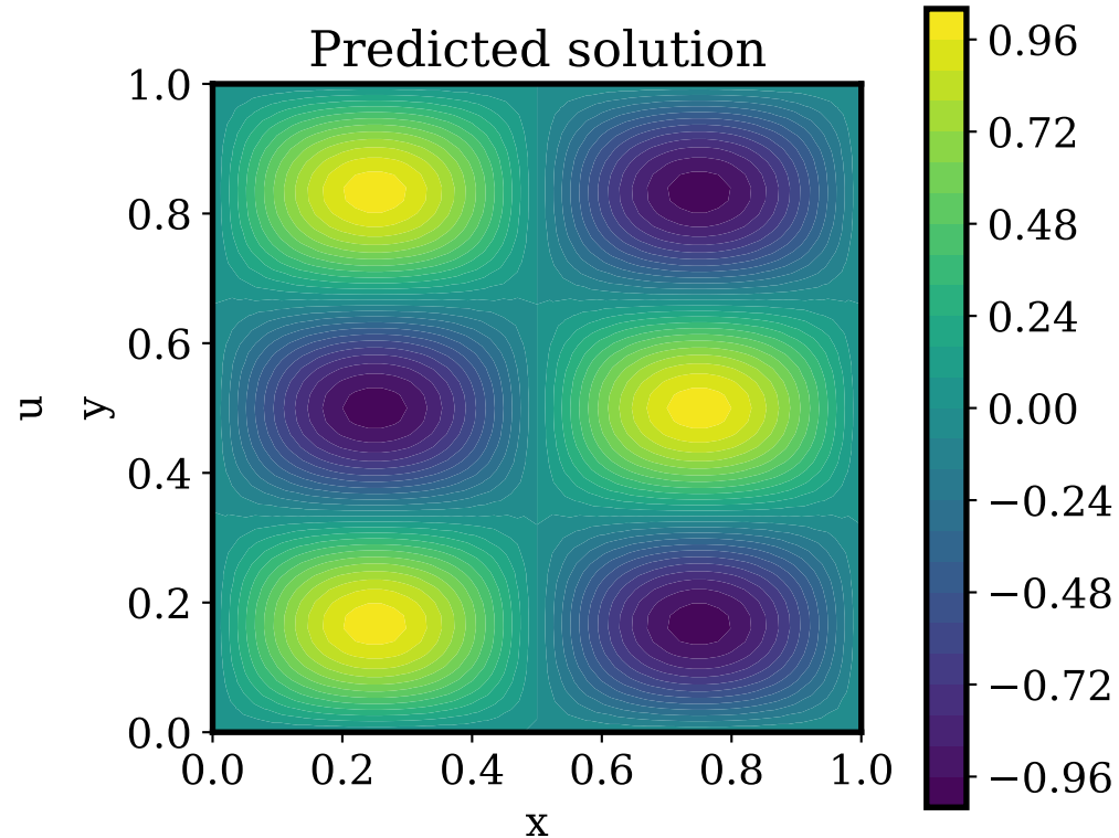
poisson: predicted vs true solution (fx=2, fy=3)
