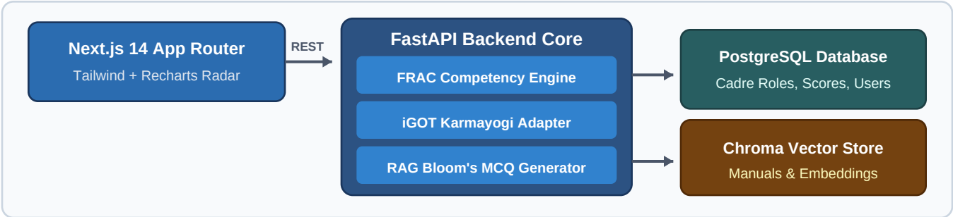
Figure 1: High-level System Architecture of DRIVYAM showing interaction between Presentation, Core Engine, and Persistence layers.
