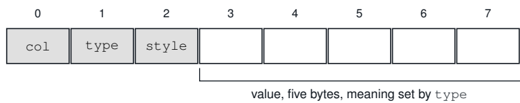
Figure B-2 The eight-byte cell record
