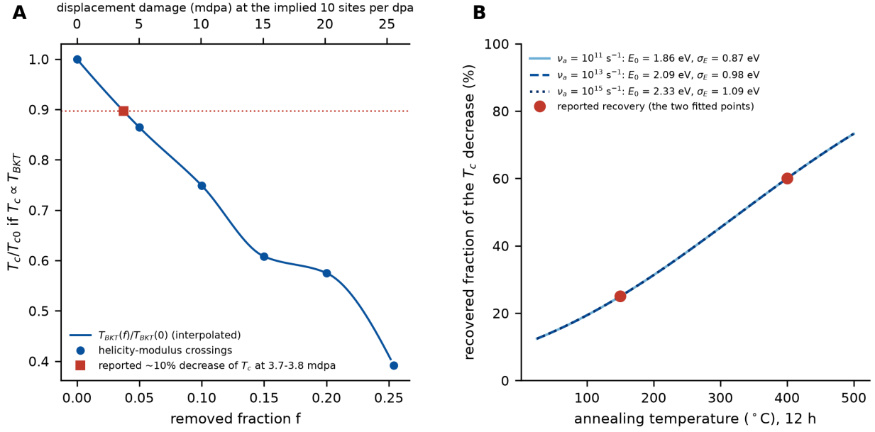
Figure 8. From damage to experiment. (a) T_c/T_{c0} = T_{BKT}(f)/T_{BKT}(0) from the helicity-modulus crossings (points, L = 16 –48 extrapolated in 1/\ln^2 L ; T_{BKT}(0) from [22]) and the interpolation used; the square marks the reported fractional decrease of T_c at 3.7–3.8 mdpa [8], which fixes the number of model sites per dpa on the upper axis. (b) Recovered fraction of the T_c decrease after 12 h anneals for a Gaussian spectrum of activation energies, fitted to the two reported recoveries [7] (points) for three attempt frequencies.
