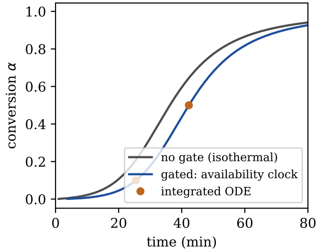
(a) Gated cure at 140 °C
