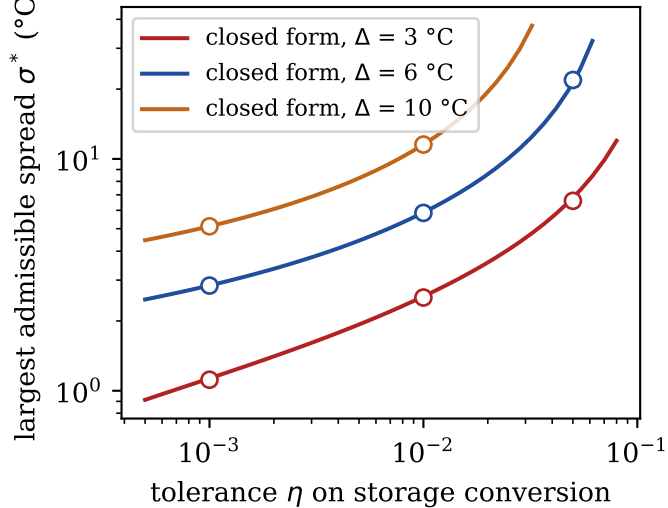
(b) Bound on the spread (open: ODE)
