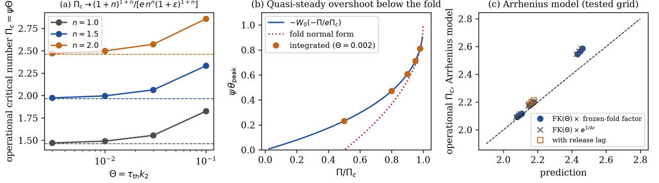
Fig. 3 (a) Operational critical number against \Theta for n = 1, 3/2 and 2 (points: integrations; dashed: finite- \varepsilon Eq. (14)). (b) Quasi-steady overshoot below \Pi_c : Lambert-W formula, fold normal form, and integrations. (c) Arrhenius operational critical number against FK(\Theta) times the frozen-fold factor.
