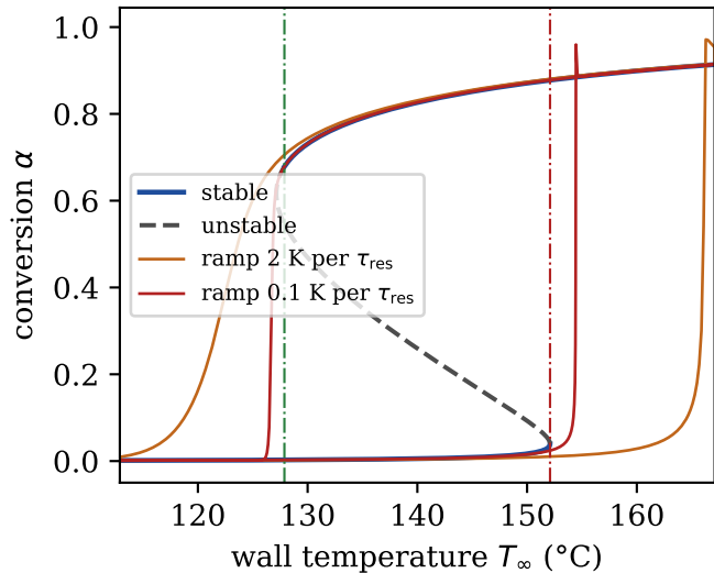
(a) Arrhenius path, \Delta T_{\text{ad}} = 220 K
