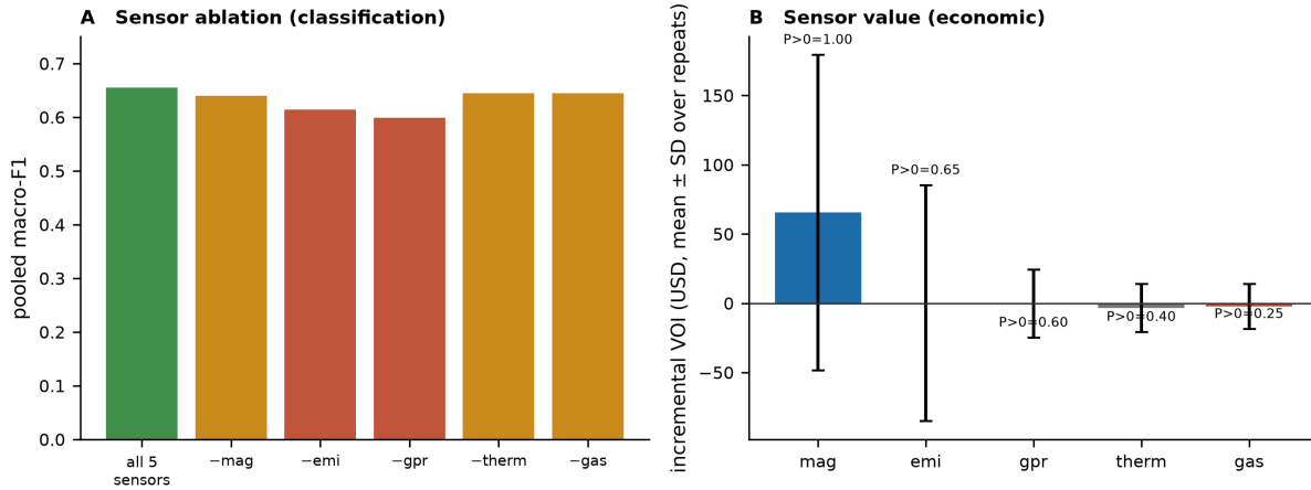
Fig. 5 (a) Pooled macro-F1 with each sensor removed in turn. (b) Incremental value of information (VOI with all sensors minus VOI without sensor j ), mean \pm SD over 20 independent surveys, with the fraction of surveys giving a positive incremental value.
