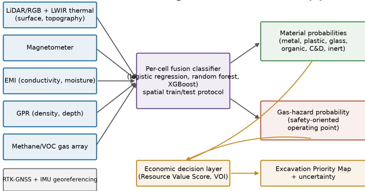
Fig. 1 LAND-MAP pipeline: co-registered sensing channels feed a per-cell fusion classifier under a spatial train/test protocol, producing material and gas-hazard probabilities that an economic decision layer converts into an excavation priority map.
