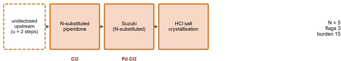
Fig. 2 Routes R0, R1 and R2 as step sequences. Box colour is the evidence class of the conditions as written; dashed boxes are the undisclosed upstream steps ( u = 2 ). Red labels are documented flags (Cl1, Cl2: ICH Q3C Class 1 and 2 solvents; Pd: palladium catalyst; HOAt: hydroxybenzotriazole-type reagent; HPLC: preparative HPLC; 2 d and 16 %: reaction time and yield of the disclosed reductive amination; lyo: lyophilisation). N is the number of steps, flags the number of flag instances and burden the validation burden on the linear scale.
