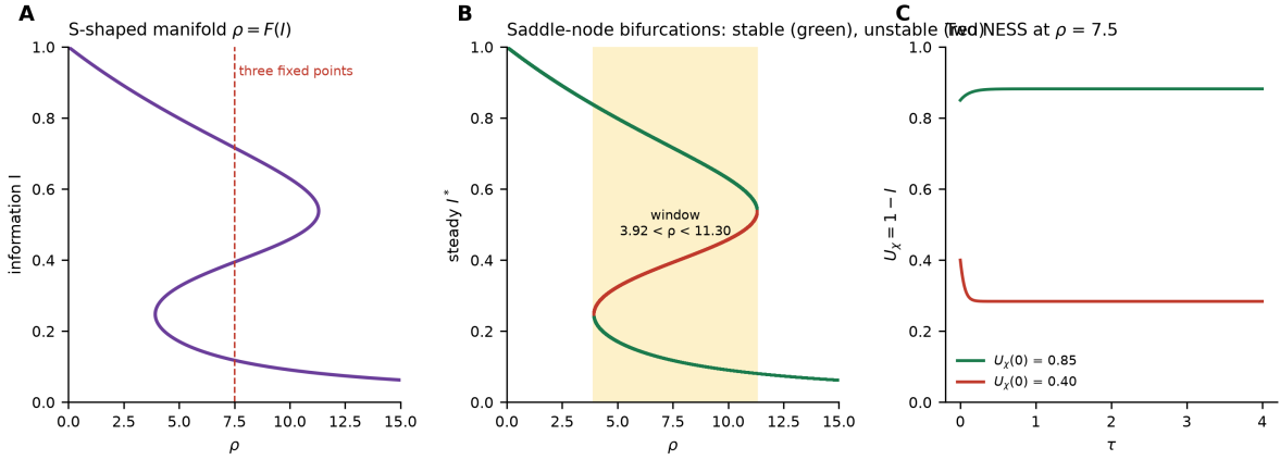
Figure 3. Nonlinear feedback \rightarrow bistability (Proposition 2). (A) The steady-state manifold \rho = F(I) is S-shaped, so a range of \rho admits three fixed points. (B) Bifurcation diagram: stable (green) and unstable (red) branches with two saddle-node points bounding a hysteresis window (shaded). (C) At \rho = 7.5 , inside the window, two initial conditions flow to a maintained and a collapsed NESS.
