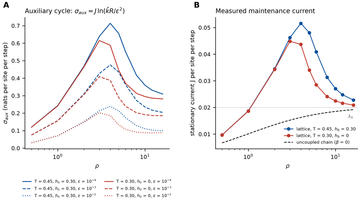
Figure 7. Maintenance current and the auxiliary cycle. (A) Entropy production rate \sigma_{\text{aux}} = J \ln(\bar{k}R/\varepsilon^2) of the auxiliary two-state cycle of Section 6 for three reverse rates \varepsilon (an illustrative, regularization-dependent quantity, not a property measured in the simulation). (B) Stationary kill current J per site and step measured in the lattice ( L = 48 , 4 runs per point; the repair current coincides) for both parameter sets, the uncoupled two-state chain (dashed) and \lambda_0 (dotted).
