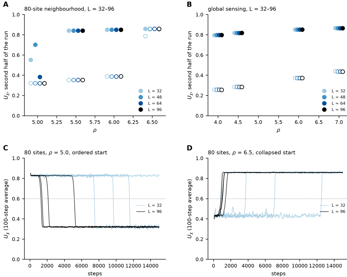
Figure A2. Extended-range bistability in size and time (4 runs per start, 15000 steps). (A, B) Order in the second half of each run from the ordered (filled) and the collapsed (open) start, for the 80-site neighbourhood and for global sensing, at L = 32-96 (points offset for visibility). (C) Ordered starts of the 80-site case at \rho = 5.0 decay to the collapsed branch, sooner at L = 96 than at L = 32 . (D) Collapsed starts at \rho = 6.5 recover. Dotted: the threshold U_X = 0.6 used to detect a switch.
