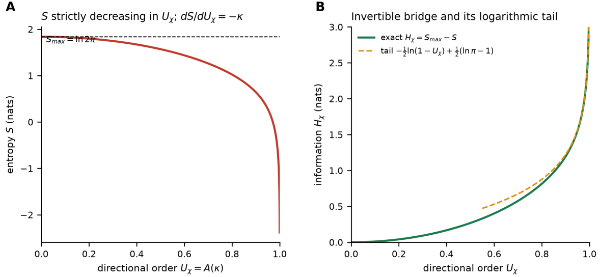
116 Figure 1. The order–entropy bridge (Theorem 1). (A) S is strictly decreasing in U_\chi . (B) H_\chi = S_{\max} - S is a strictly 117 increasing invertible image of U_\chi , with the derived logarithmic tail (dashed).
