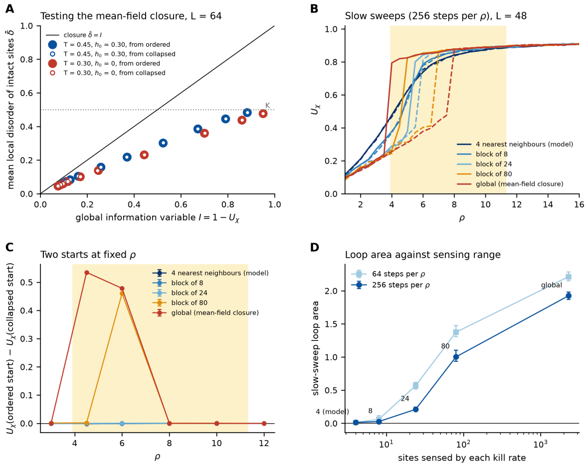
Figure 5. Why nearest-neighbour feedback is not bistable, and the sensing range that restores bistability. (A) Mean local disorder of intact sites \bar{\delta} against the global I = 1 - U_x in the stationary lattice ( L = 64 ; filled: ordered start, open: collapsed start; both parameter sets); the line is the closure \bar{\delta} = I and the dotted line marks K . (B) Slow sweeps (256 steps per \rho value) at L = 48 with the kill rate sensing the 4 nearest neighbours (the model), blocks of 8, 24 and 80 sites, or the global disorder; solid down, dashed up; the mean-field window is shaded. (C) Difference in stationary order between the ordered and the collapsed start at fixed \rho , with 95% intervals. (D) Slow-sweep loop area against the number of sites sensed, at 64 and 256 steps per \rho value.
