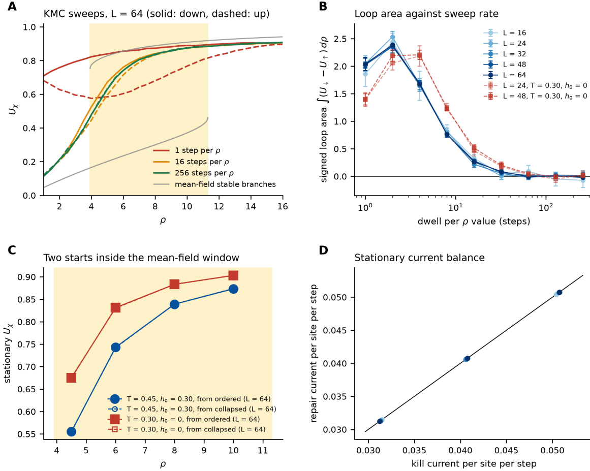
211 Figure 4. Kinetic Monte Carlo test of Proposition 2 on the nearest-neighbour lattice ( T = 0.45 , h_0 = 0.30 unless 212 stated). (A) Sweeps of \rho down (solid) and up (dashed) at L = 64 , with 1, 16 and 256 steps per \rho value: the loop of 213 fast sweeps closes as the sweep slows; the mean-field window is shaded and its stable branches are grey. (B) Signed 214 loop area against dwell per \rho value for L = 16 – 64 and for the colder field-free variant (squares); mean \pm 95% 215 interval over 8 runs. (C) Stationary order from an ordered and a collapsed start at fixed \rho inside the window ( L = 216 64 ): the two coincide. (D) Stationary kill and repair currents per site and step at \rho = 4.5, 6 and 8 and L = 16, 32, 64 ; 217 the line is equality.
