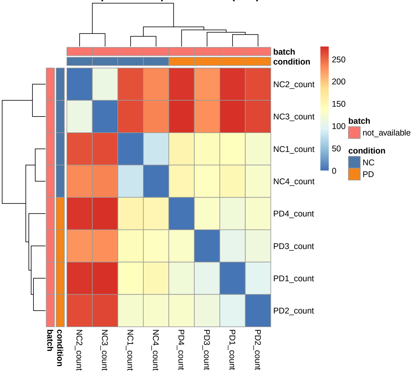
Sample-to-sample distances (VST)
