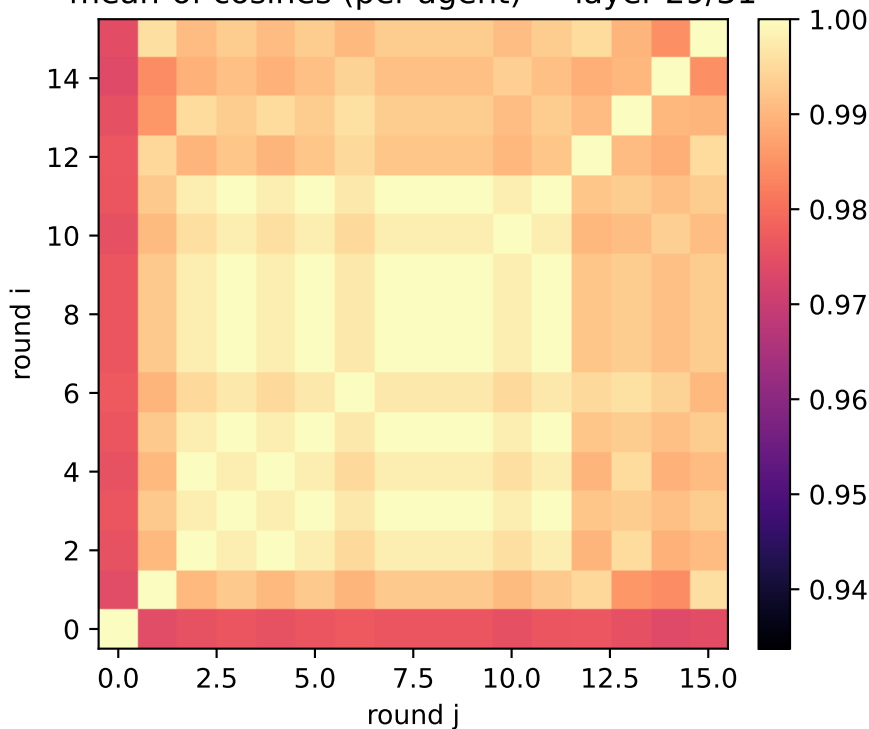
exp1: detailed clues (two_layer) mean-of-cosines (per-agent) — layer 29/31
