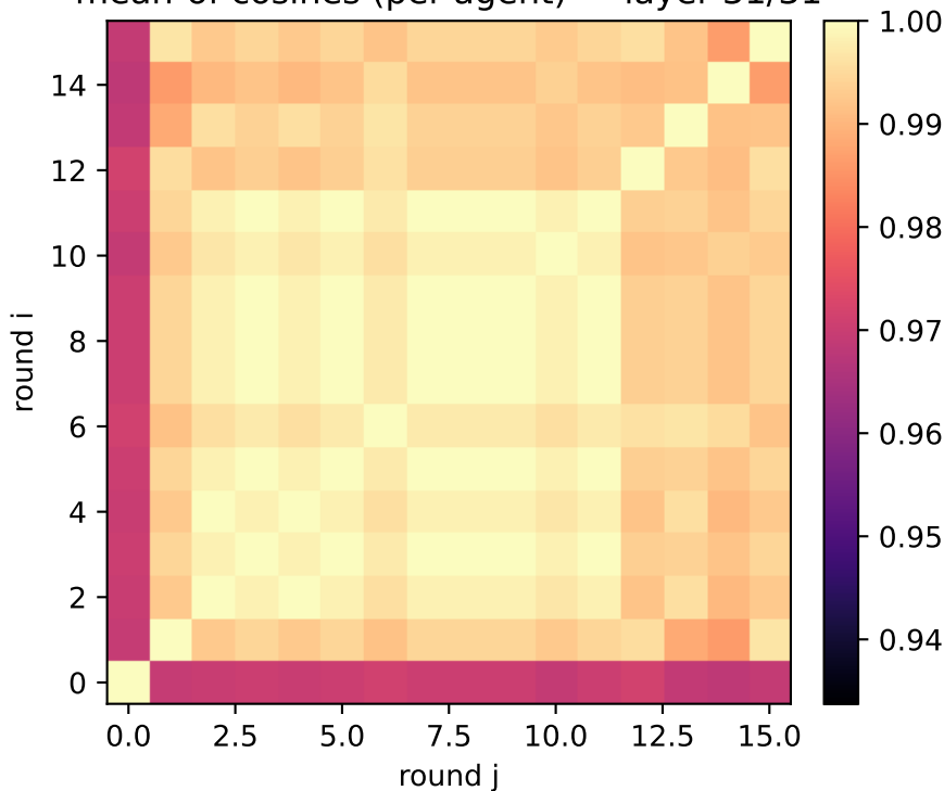
exp1: detailed clues (two_layer) mean-of-cosines (per-agent) — layer 31/31
