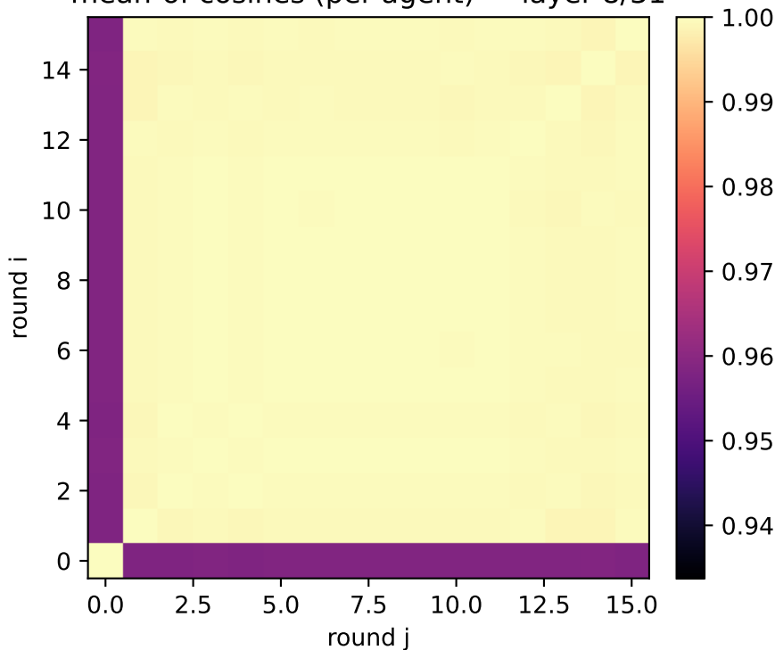
exp1: detailed clues (two_layer) mean-of-cosines (per-agent) — layer 8/31
