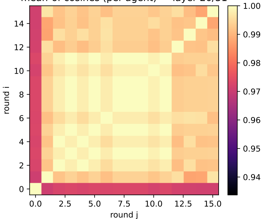
exp1: detailed clues (two_layer) mean-of-cosines (per-agent) — layer 20/31
