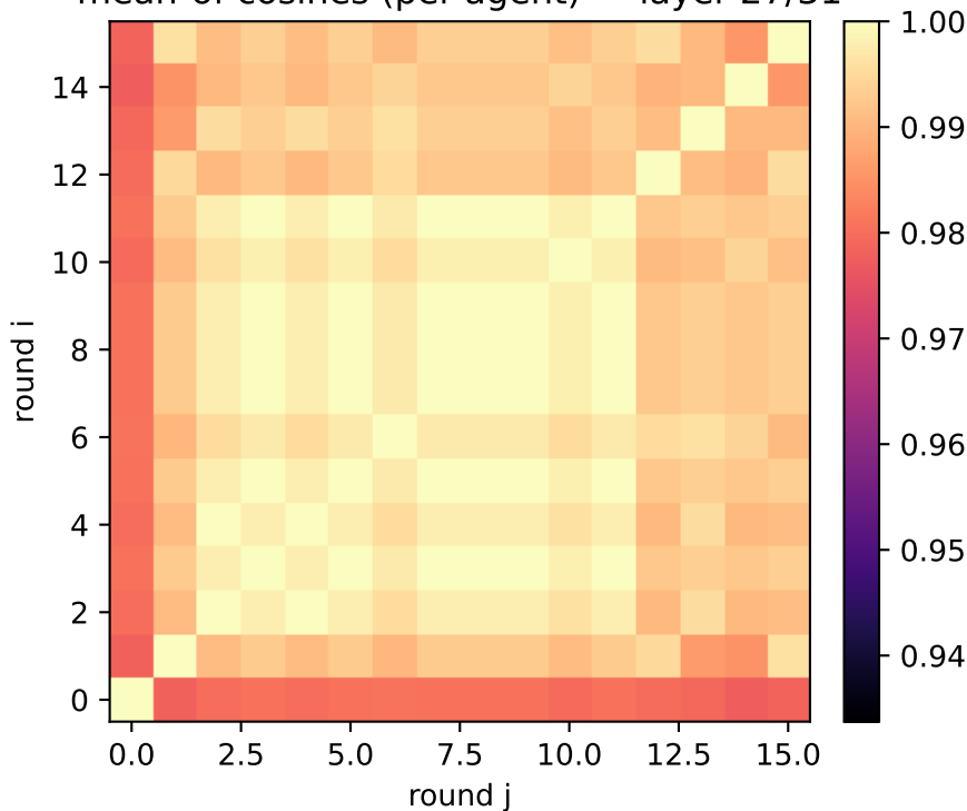
exp1: detailed clues (two_layer) mean-of-cosines (per-agent) — layer 27/31
