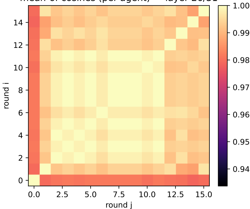
exp1: detailed clues (two_layer) mean-of-cosines (per-agent) — layer 26/31
