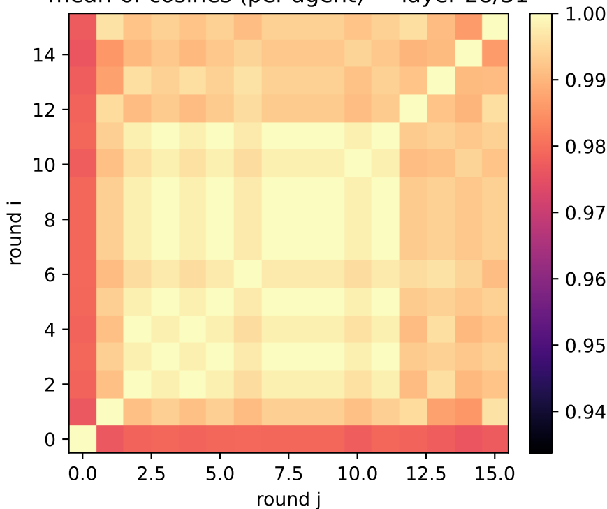
exp1: detailed clues (two_layer) mean-of-cosines (per-agent) — layer 28/31
