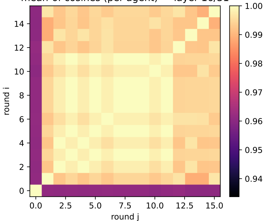
exp1: detailed clues (two_layer) mean-of-cosines (per-agent) — layer 16/31
