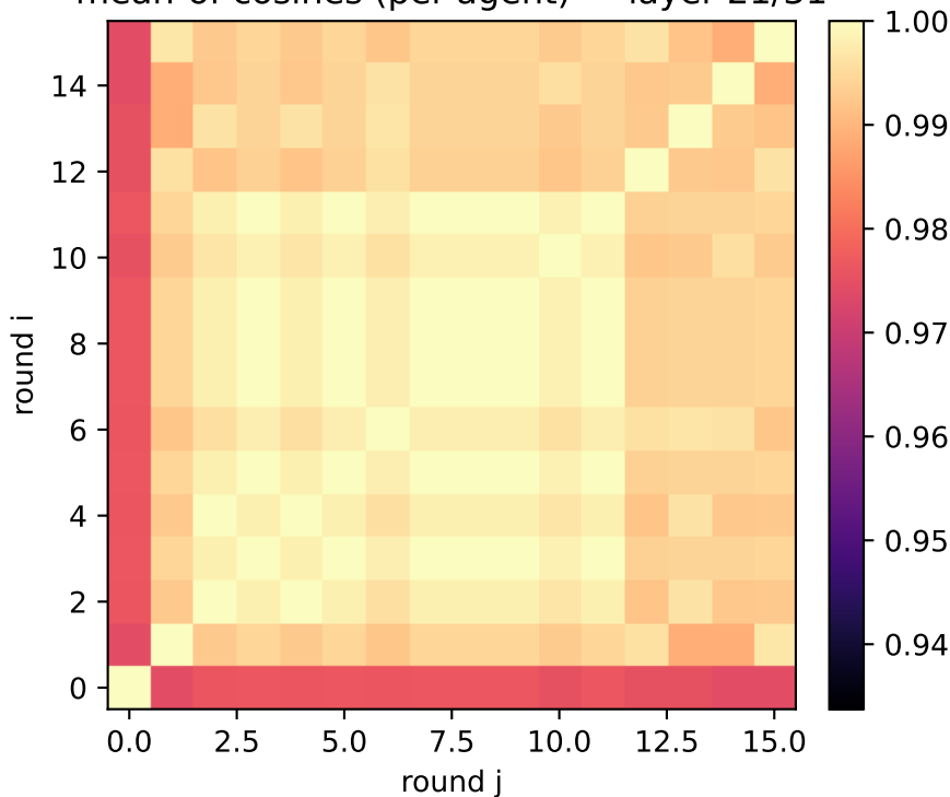
exp1: detailed clues (two_layer) mean-of-cosines (per-agent) — layer 21/31
