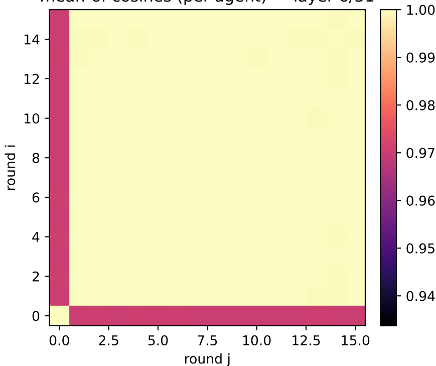
exp1: detailed clues (two_layer) mean-of-cosines (per-agent) — layer 6/31
