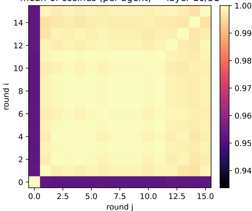
exp1: detailed clues (two_layer) mean-of-cosines (per-agent) — layer 10/31
