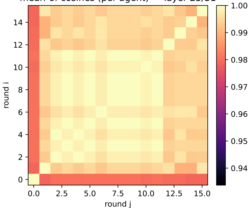
exp1: detailed clues (two_layer) mean-of-cosines (per-agent) — layer 23/31
