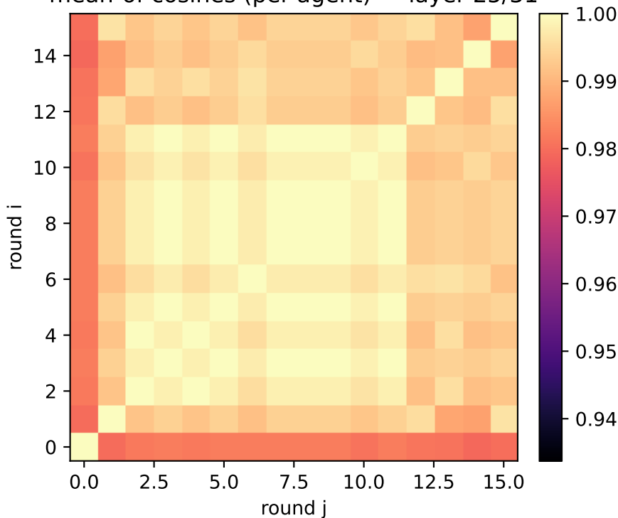
exp1: detailed clues (two_layer) mean-of-cosines (per-agent) — layer 25/31
