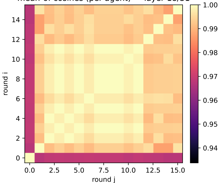
exp1: detailed clues (two_layer) mean-of-cosines (per-agent) — layer 18/31
