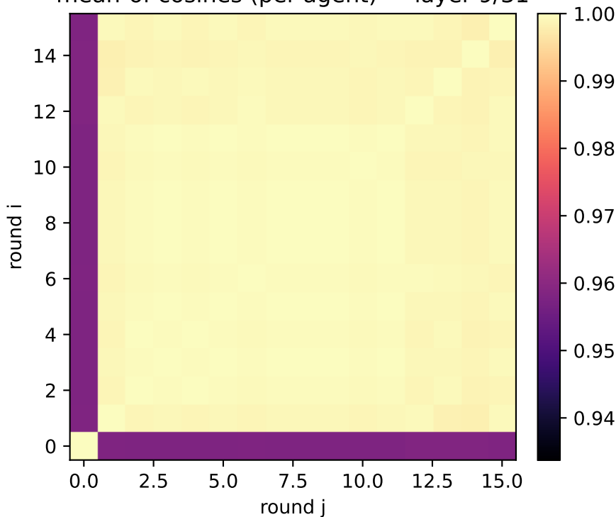
exp1: detailed clues (two_layer) mean-of-cosines (per-agent) — layer 9/31
