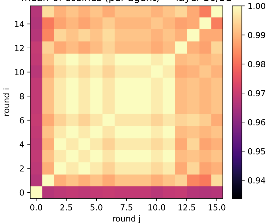
exp1: detailed clues (two_layer) mean-of-cosines (per-agent) — layer 30/31
