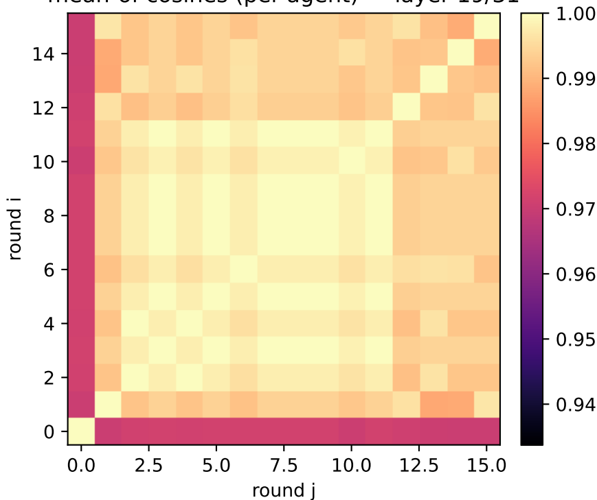
exp1: detailed clues (two_layer) mean-of-cosines (per-agent) — layer 19/31
