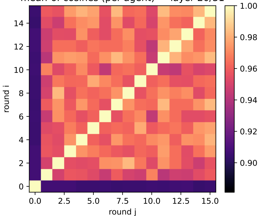
exp2: generic attributes (two_layer) mean-of-cosines (per-agent) — layer 20/31
