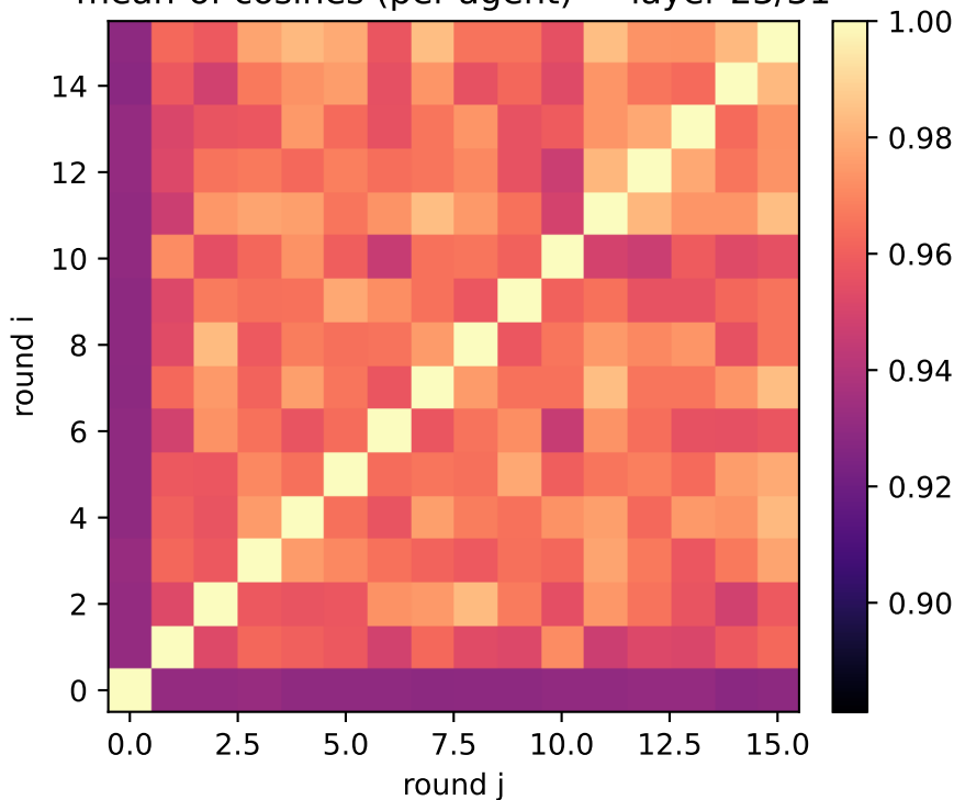
exp2: generic attributes (two_layer) mean-of-cosines (per-agent) — layer 23/31
