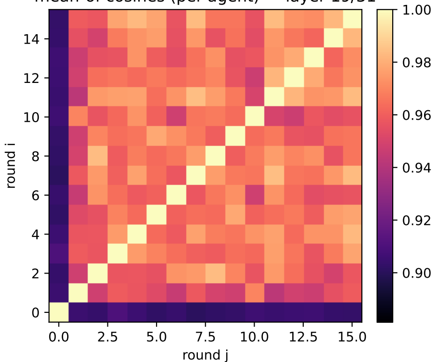
exp2: generic attributes (two_layer) mean-of-cosines (per-agent) — layer 19/31
