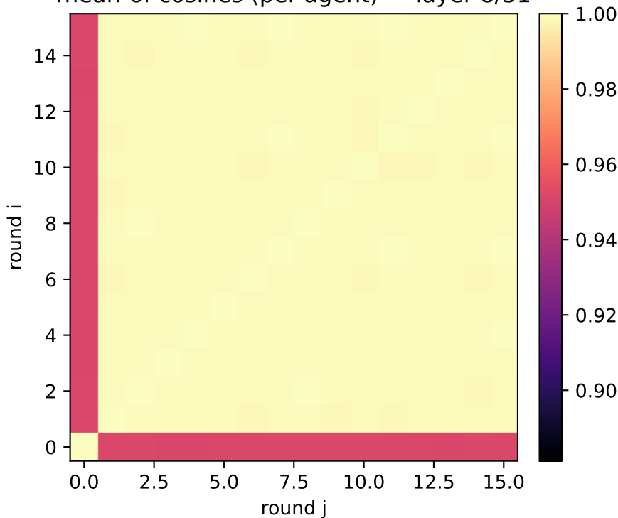
exp2: generic attributes (two_layer) mean-of-cosines (per-agent) — layer 8/31
