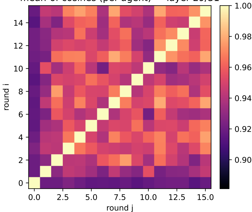
exp2: generic attributes (two_layer) mean-of-cosines (per-agent) — layer 29/31
