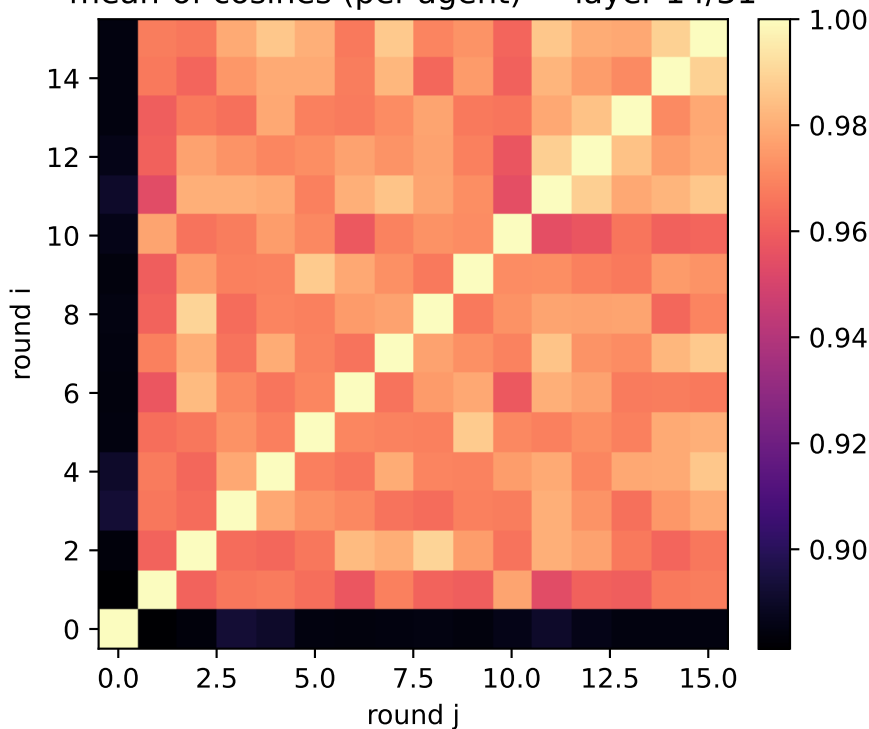
exp2: generic attributes (two_layer) mean-of-cosines (per-agent) — layer 14/31
