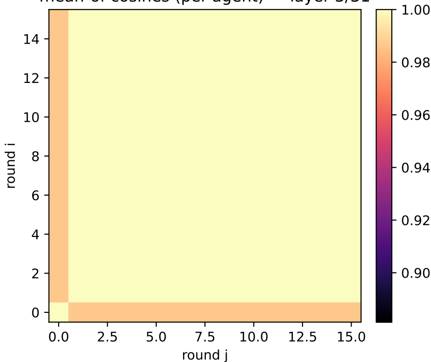
exp2: generic attributes (two_layer) mean-of-cosines (per-agent) — layer 3/31
