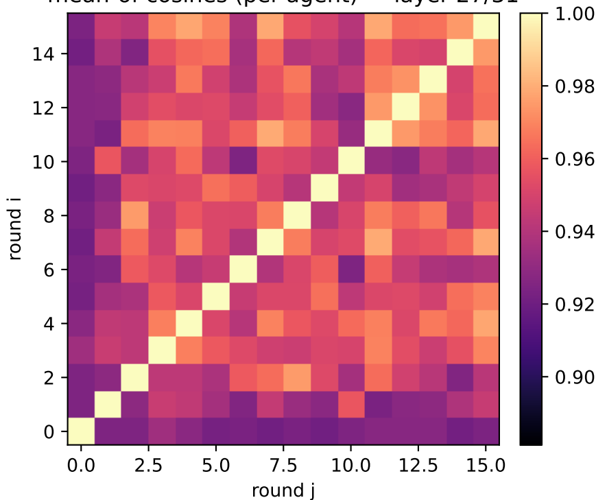
exp2: generic attributes (two_layer) mean-of-cosines (per-agent) — layer 27/31
