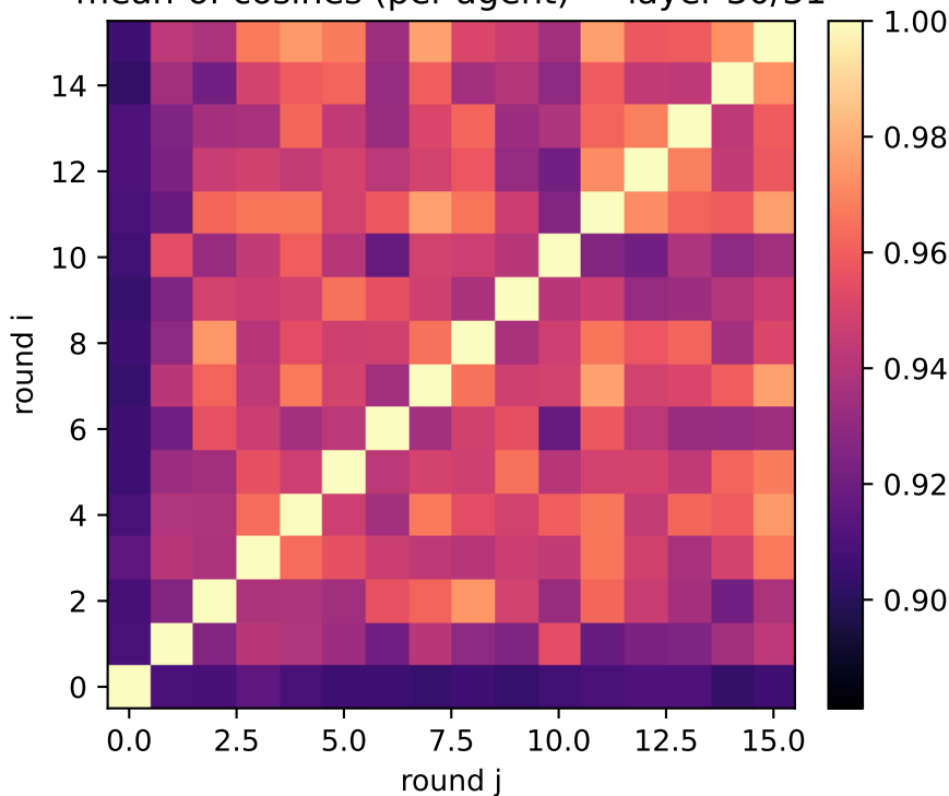
exp2: generic attributes (two_layer) mean-of-cosines (per-agent) — layer 30/31
