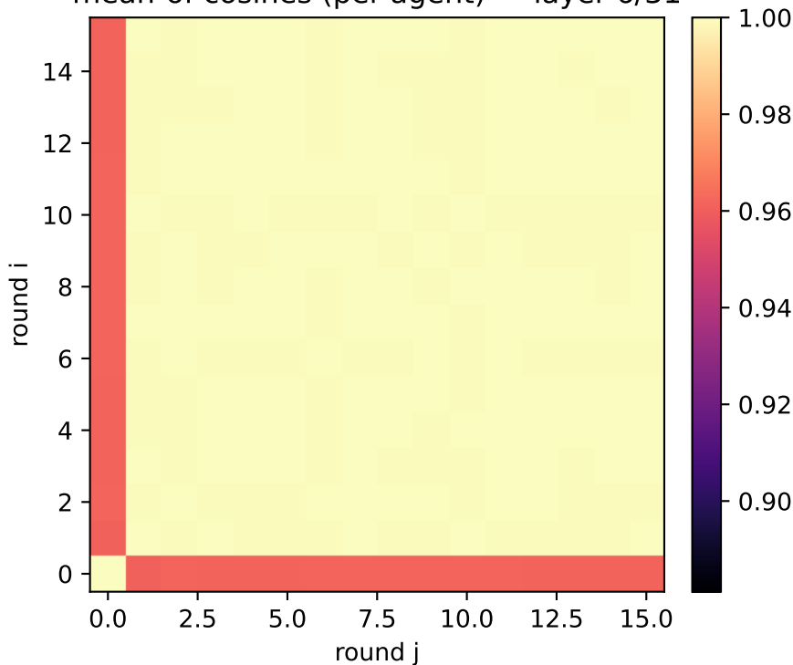
exp2: generic attributes (two_layer) mean-of-cosines (per-agent) — layer 6/31
