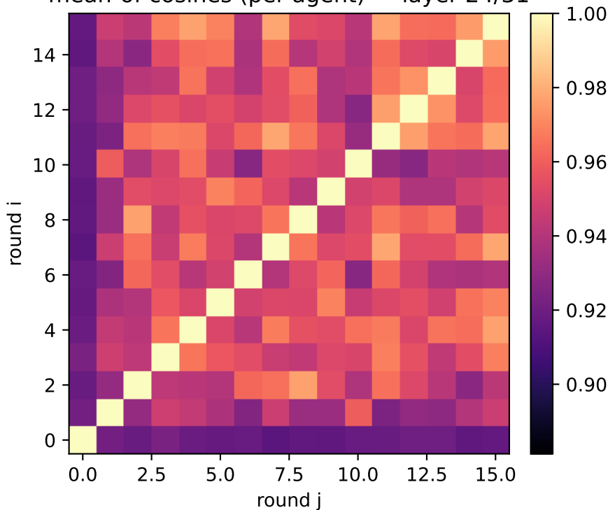
exp2: generic attributes (two_layer) mean-of-cosines (per-agent) — layer 24/31
