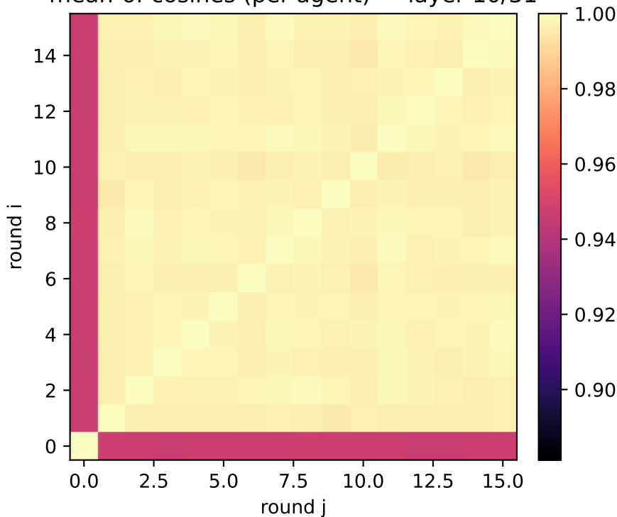
exp2: generic attributes (two_layer) mean-of-cosines (per-agent) — layer 10/31
