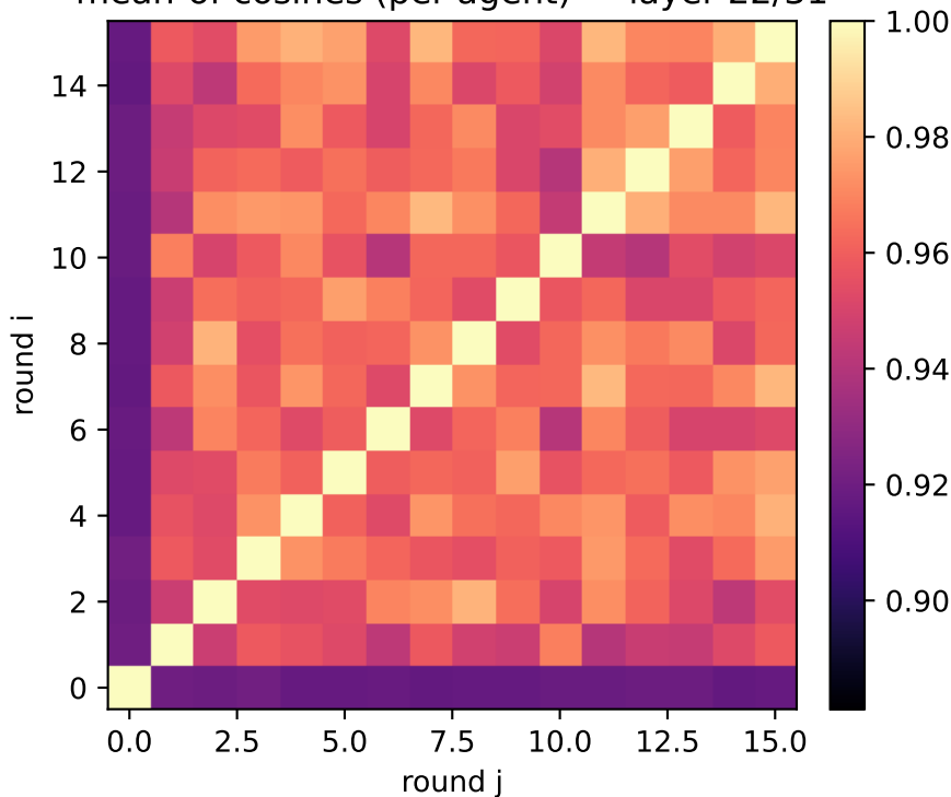
exp2: generic attributes (two_layer) mean-of-cosines (per-agent) — layer 22/31
