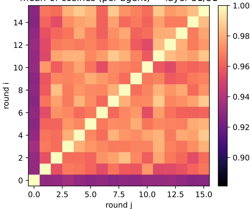
exp2: generic attributes (two_layer) mean-of-cosines (per-agent) — layer 31/31
