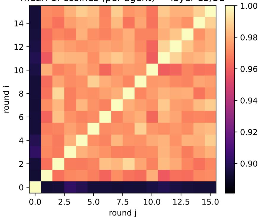
exp2: generic attributes (two_layer) mean-of-cosines (per-agent) — layer 15/31
