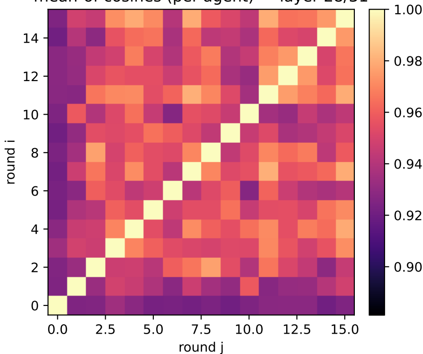
exp2: generic attributes (two_layer) mean-of-cosines (per-agent) — layer 28/31
