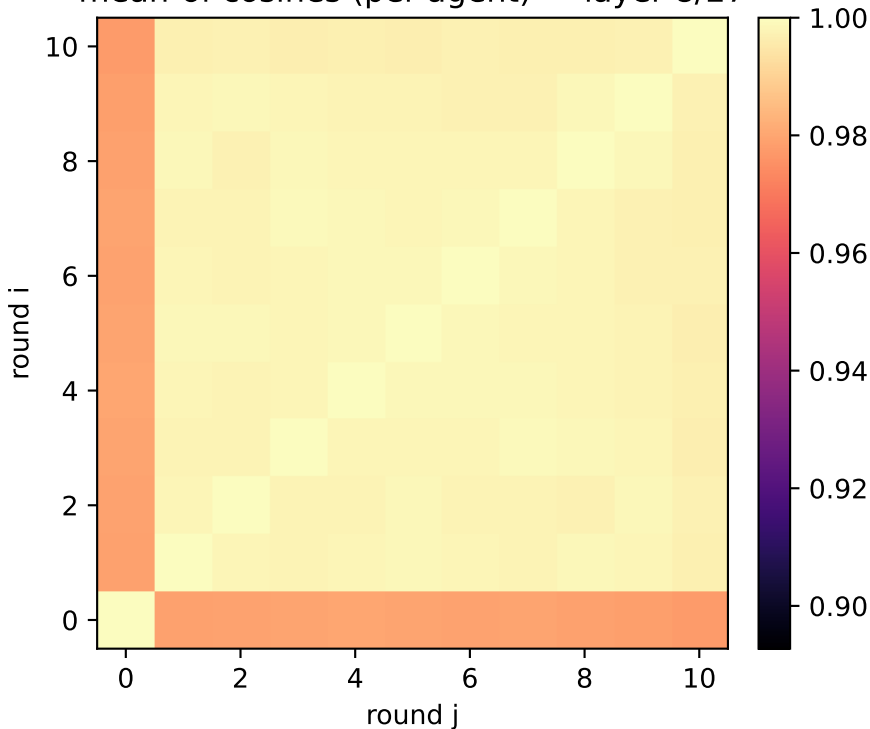
image: elephant patches (Qwen2-VL) mean-of-cosines (per-agent) — layer 8/27
