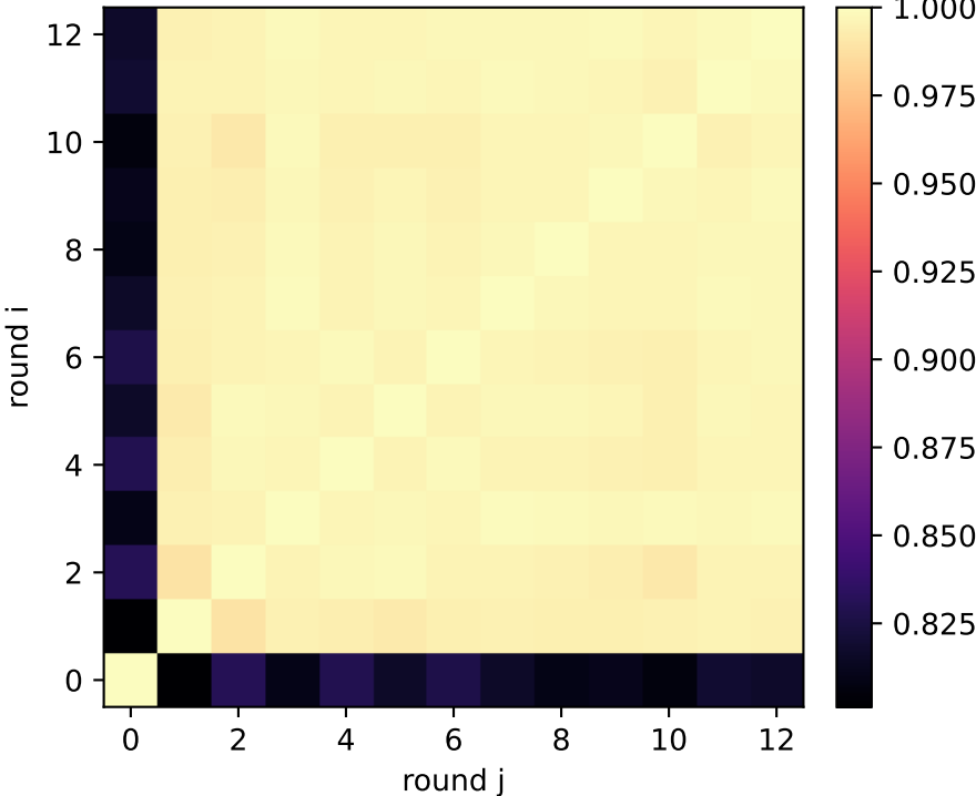
talk: QSG reasoning exchange activation similarity — layer 13/31
