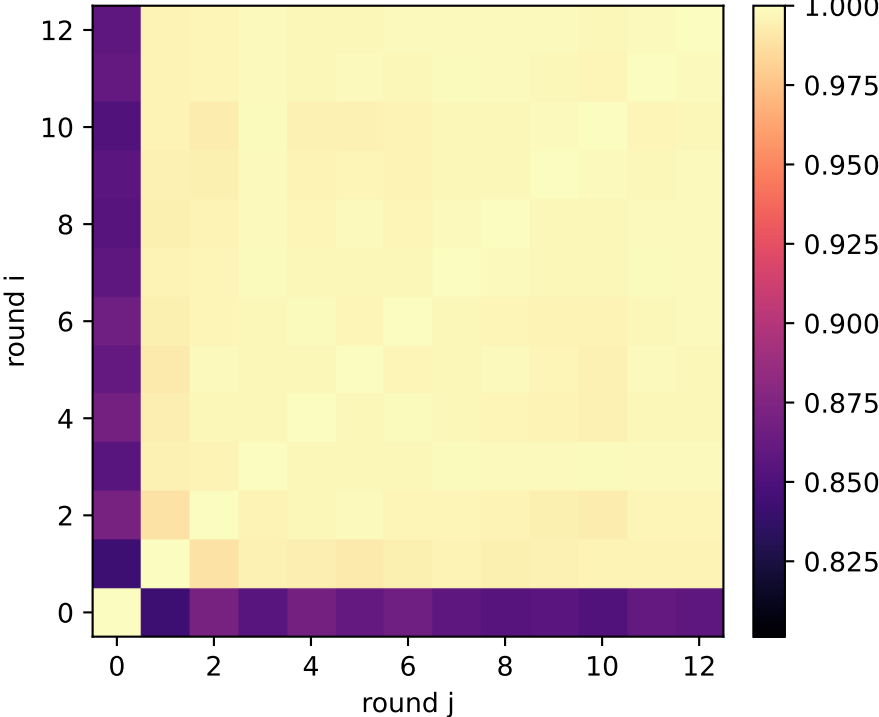
talk: QSG reasoning exchange activation similarity — layer 12/31
