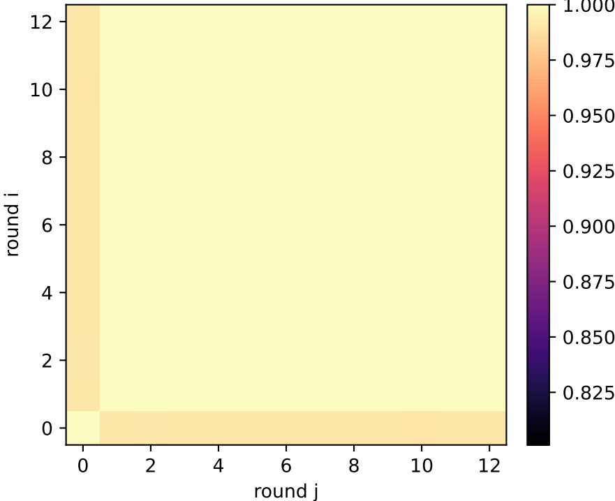
talk: QSG reasoning exchange activation similarity — layer 1/31
