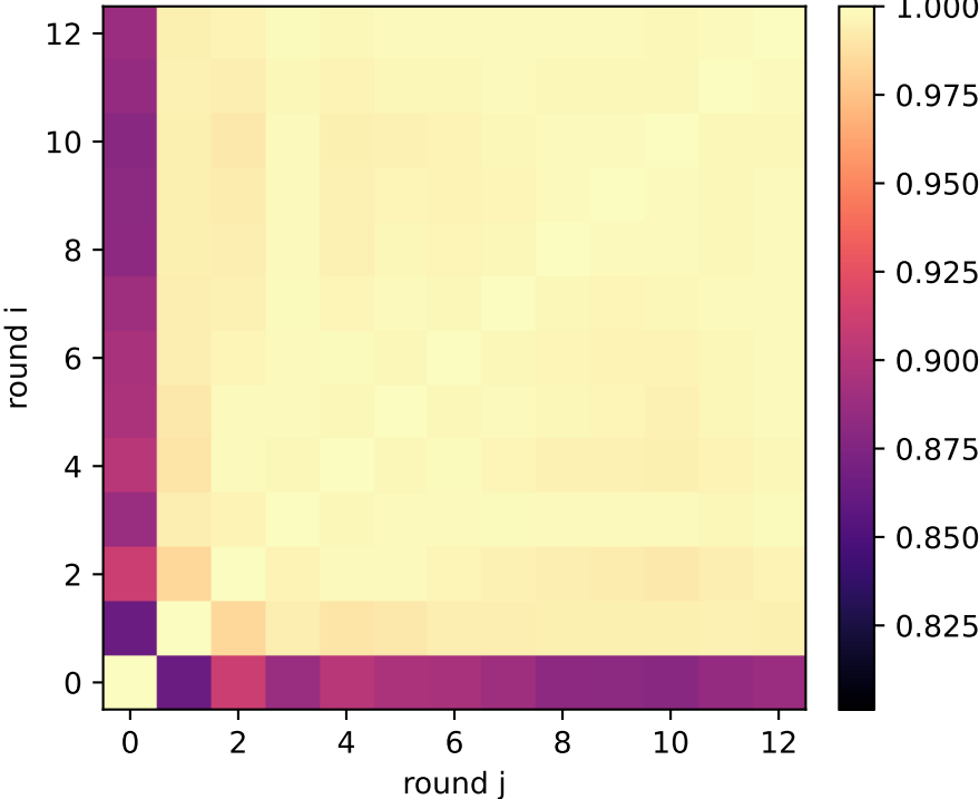
talk: QSG reasoning exchange activation similarity — layer 21/31
