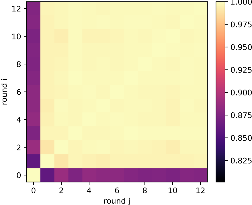
talk: QSG reasoning exchange activation similarity — layer 11/31
