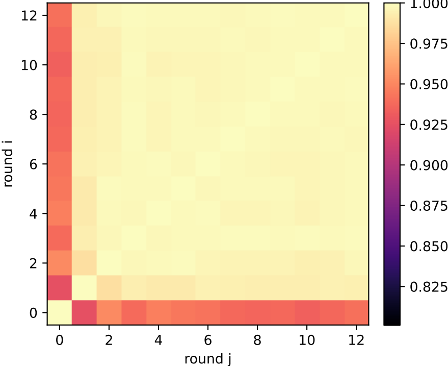
talk: QSG reasoning exchange activation similarity — layer 26/31
