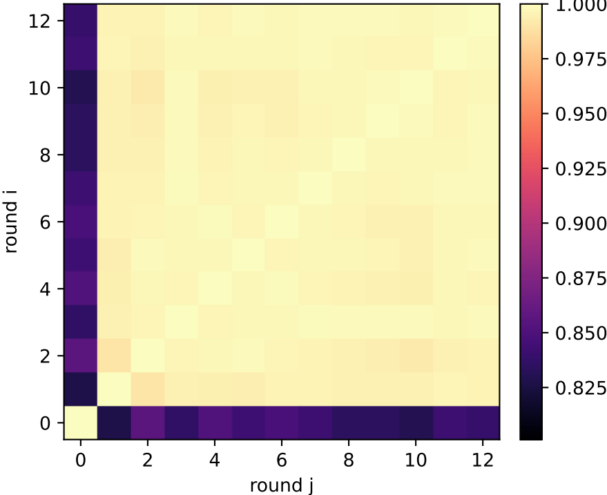
talk: QSG reasoning exchange activation similarity — layer 15/31
