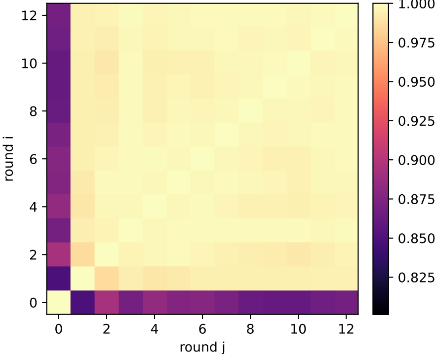
talk: QSG reasoning exchange activation similarity — layer 20/31
