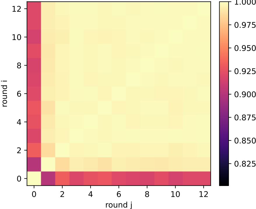
talk: QSG reasoning exchange activation similarity — layer 31/31
