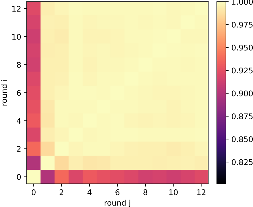
talk: QSG reasoning exchange activation similarity — layer 23/31
