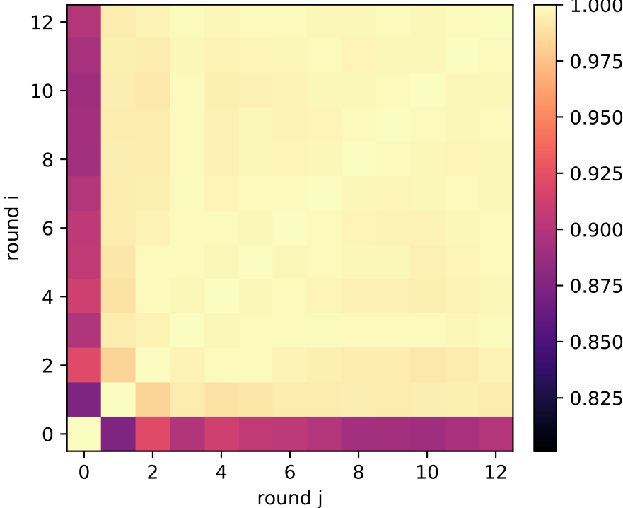
talk: QSG reasoning exchange activation similarity — layer 22/31
