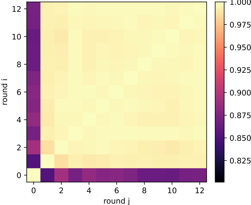
talk: QSG reasoning exchange activation similarity — layer 19/31
