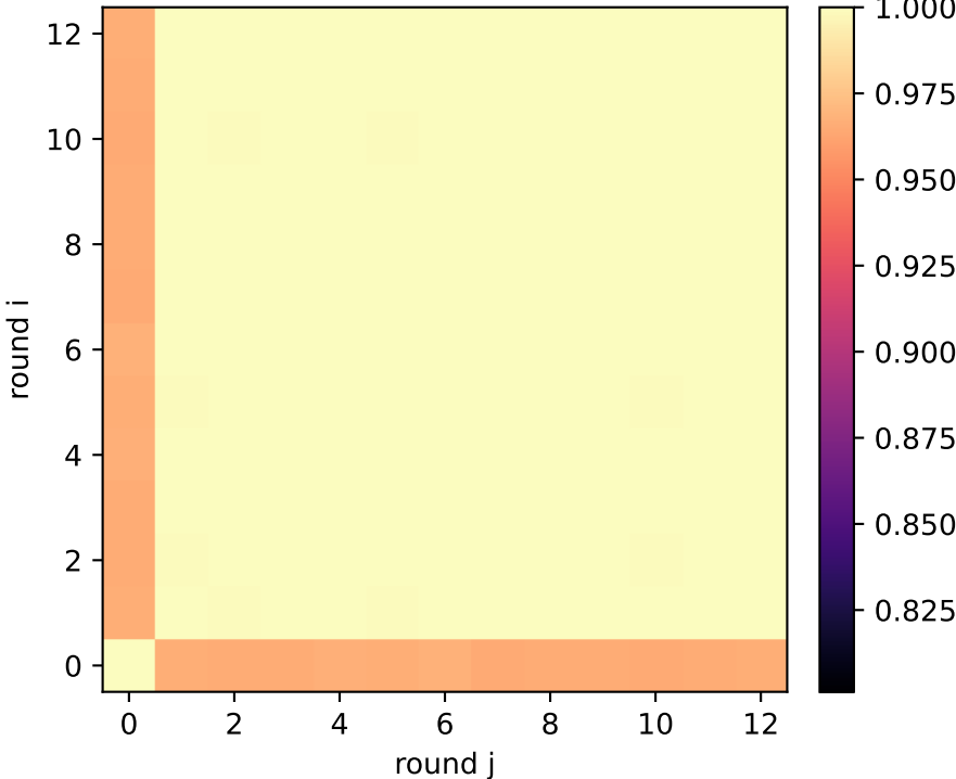
talk: QSG reasoning exchange activation similarity — layer 4/31
