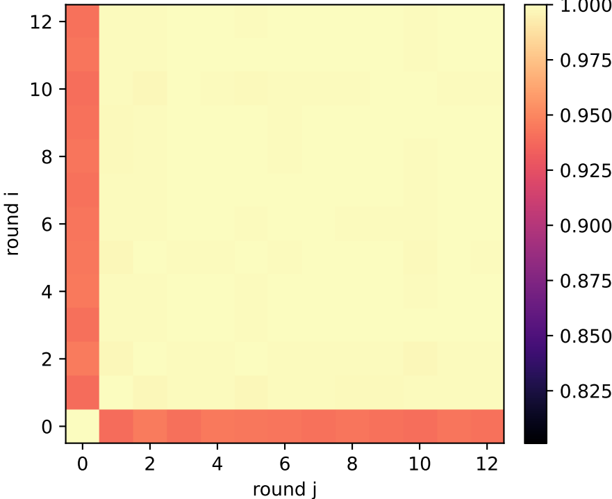
talk: QSG reasoning exchange activation similarity — layer 7/31
