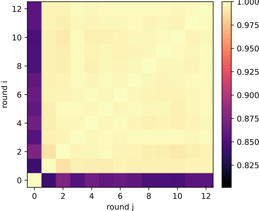
talk: QSG reasoning exchange activation similarity — layer 17/31
