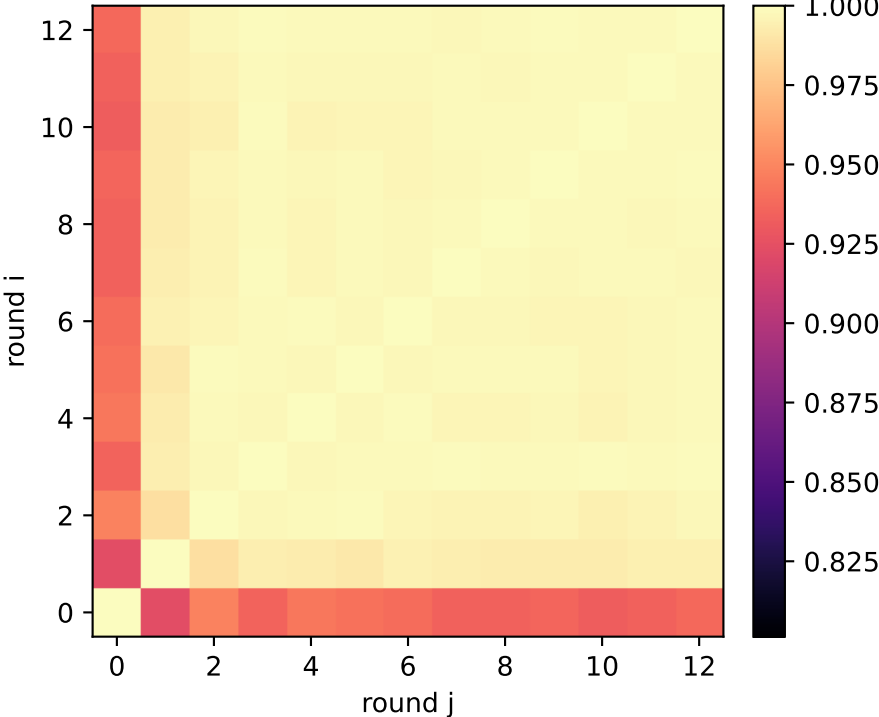
talk: QSG reasoning exchange activation similarity — layer 28/31
