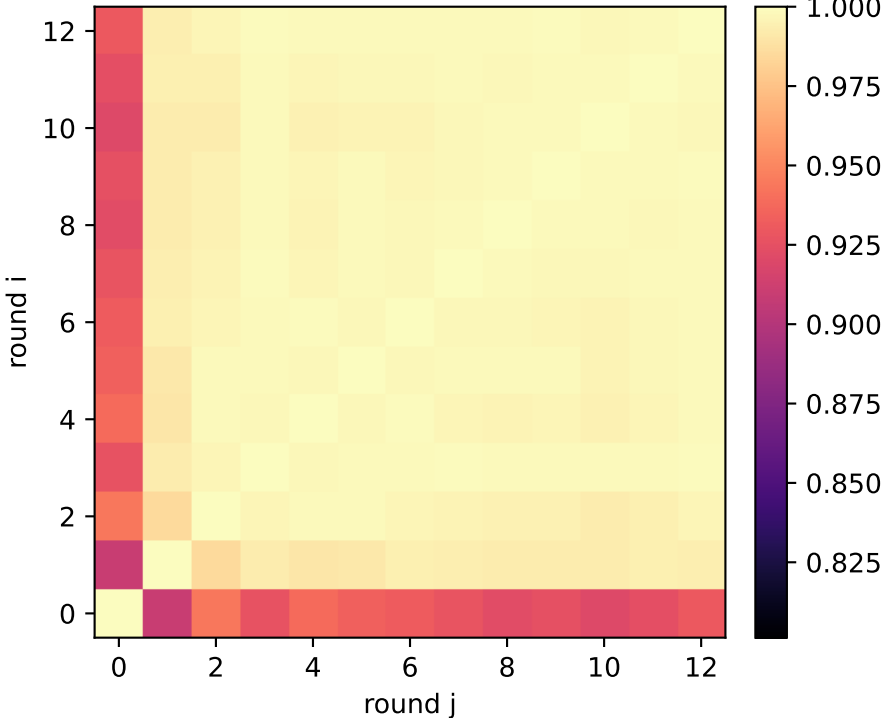
talk: QSG reasoning exchange activation similarity — layer 24/31
