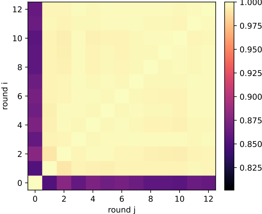
talk: QSG reasoning exchange activation similarity — layer 16/31
