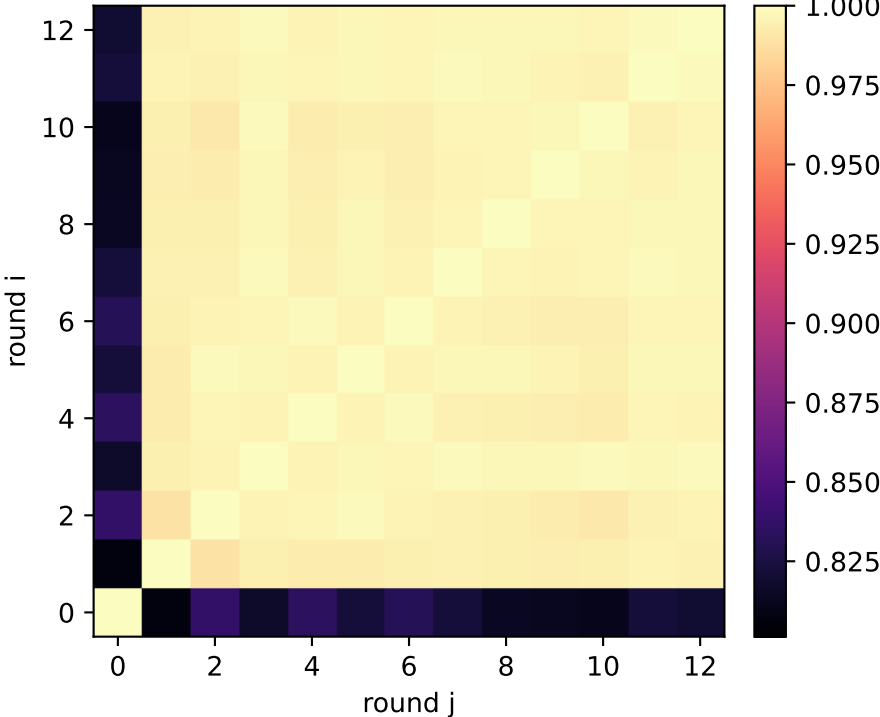
talk: QSG reasoning exchange activation similarity — layer 14/31
