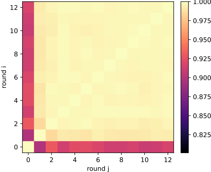
talk: QSG reasoning exchange activation similarity — layer 30/31
