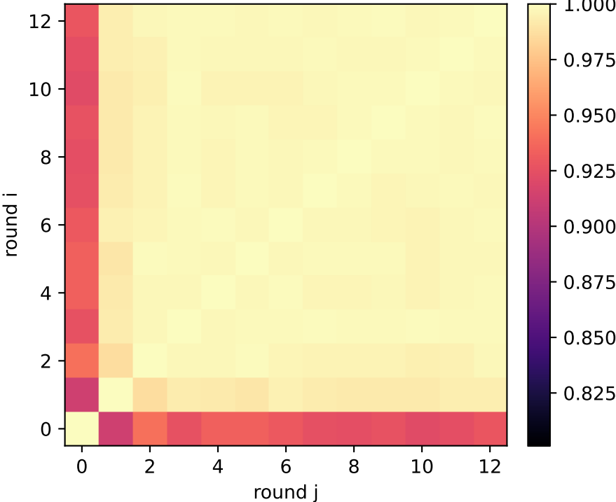
talk: QSG reasoning exchange activation similarity — layer 29/31
