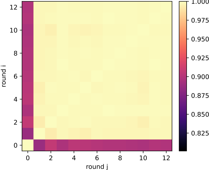
talk: QSG reasoning exchange activation similarity — layer 10/31
