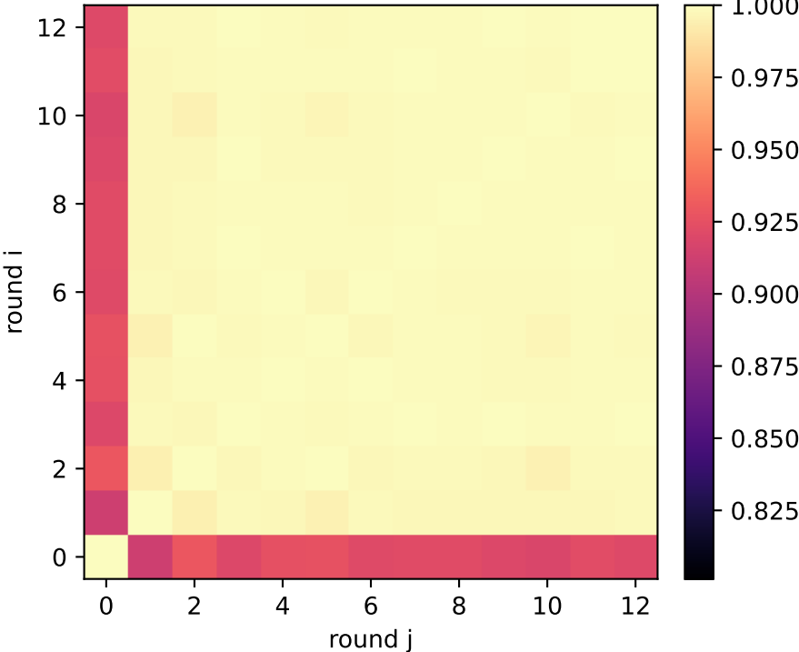
talk: QSG reasoning exchange activation similarity — layer 9/31
