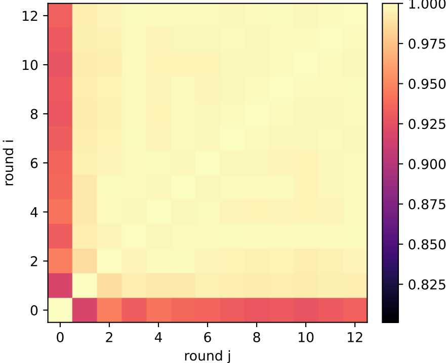
talk: QSG reasoning exchange activation similarity — layer 25/31
