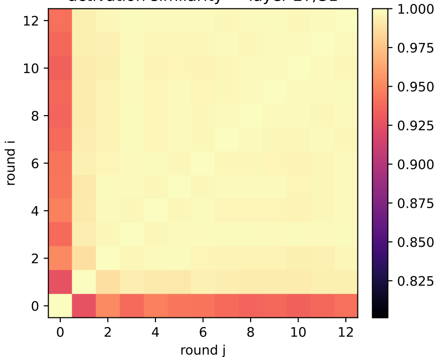
talk: QSG reasoning exchange activation similarity — layer 27/31
