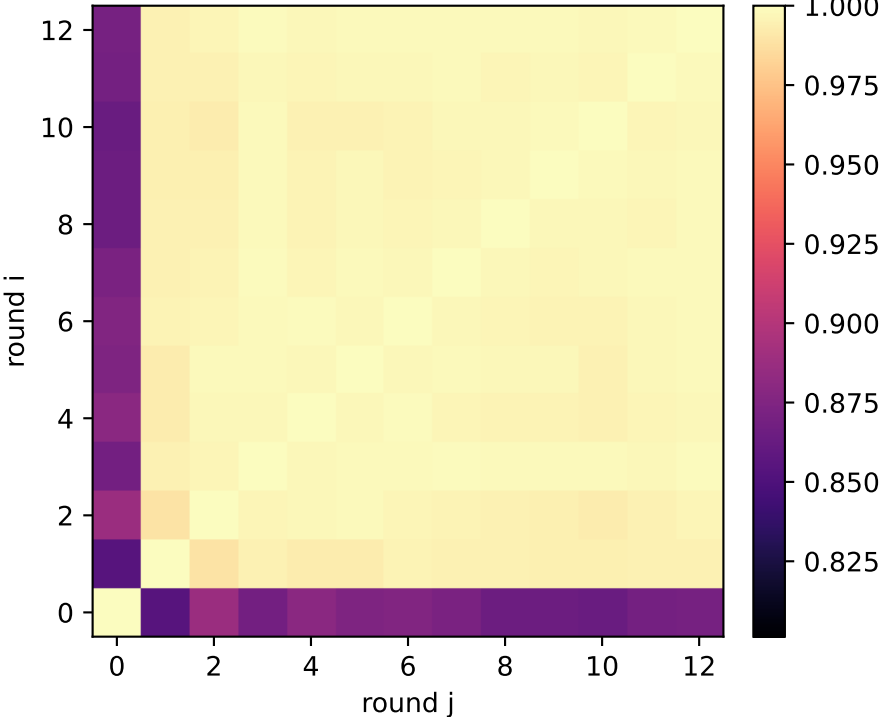
talk: QSG reasoning exchange activation similarity — layer 18/31
