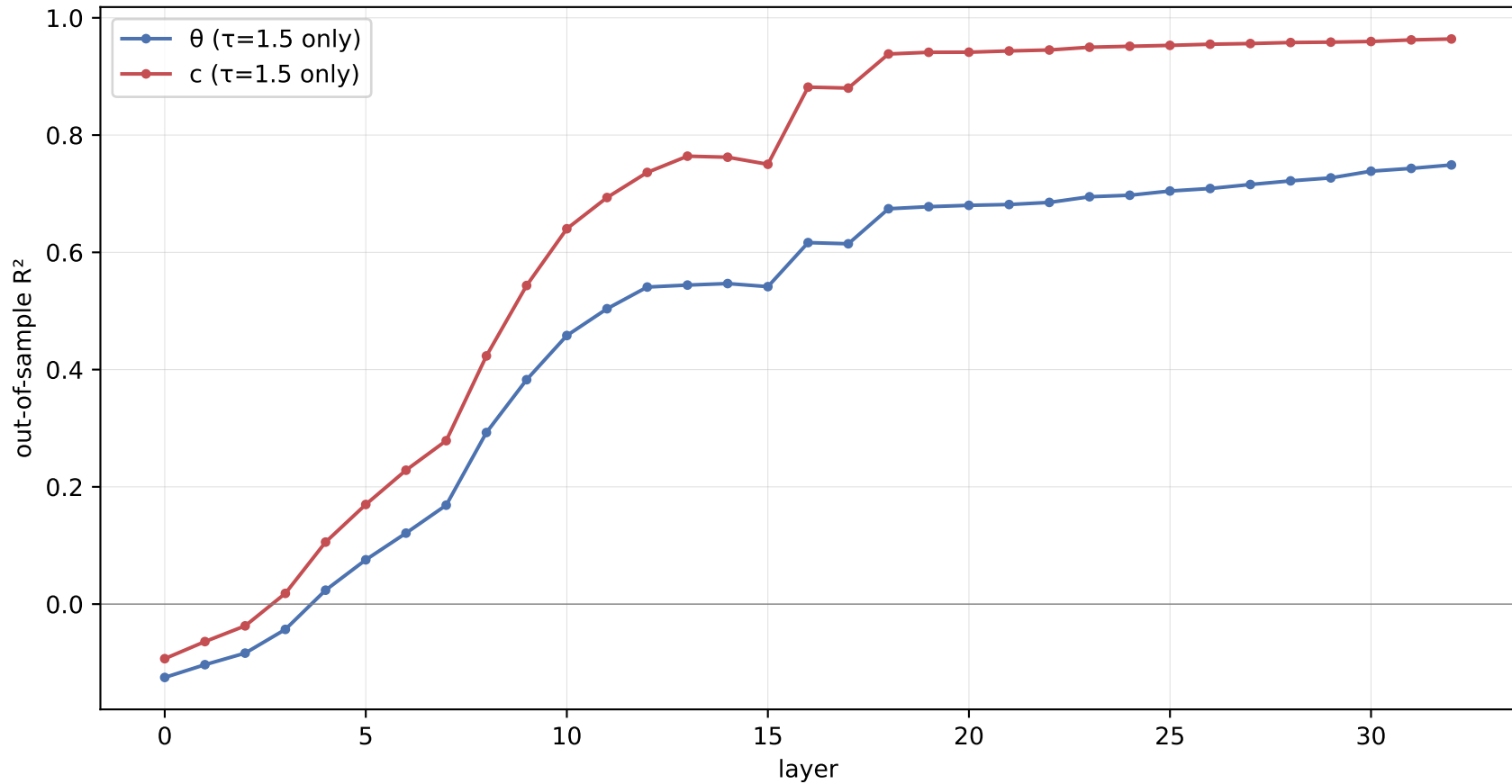
scoped: \theta vs c when they differ ( \tau=1.5 subset)
