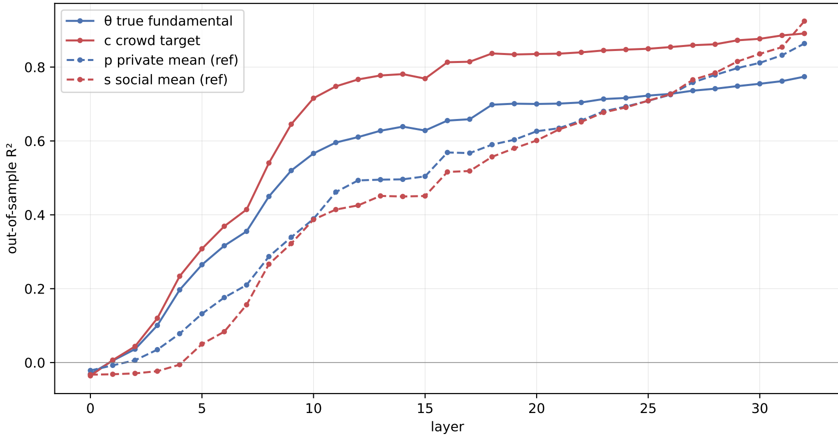
scoped: decoding TRUE latents ( \theta , c ) vs observable means ( p , s )
