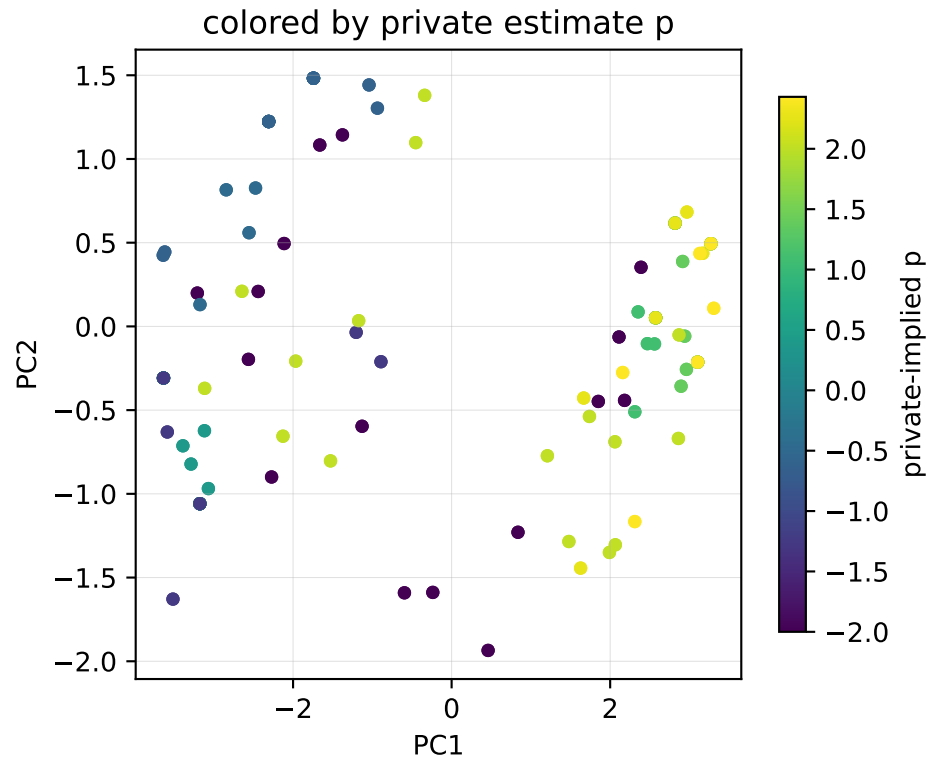
Layer 30/32 — PCA of marker activations (PC1 75.3% / PC2 7.5% variance)
