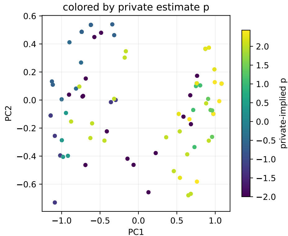
Layer 20/32 — PCA of marker activations (PC1 68.9% / PC2 10.8% variance)
