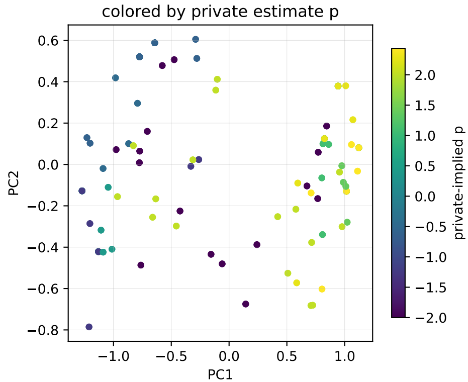
Layer 21/32 — PCA of marker activations (PC1 69.9% / PC2 10.6% variance)
