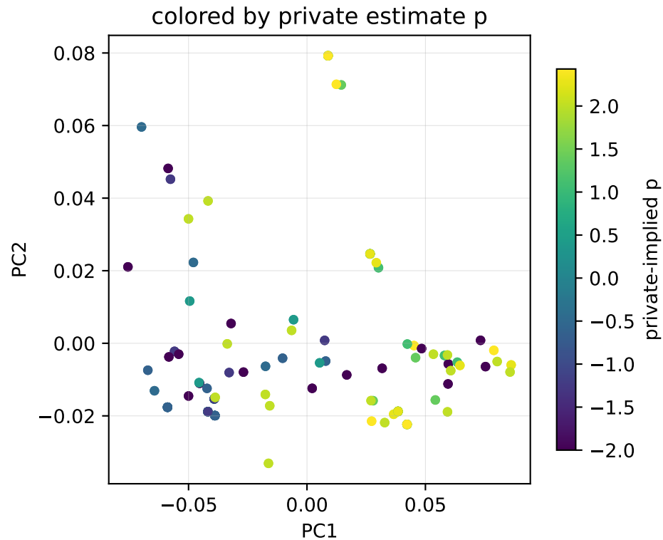
Layer 5/32 — PCA of marker activations (PC1 40.3% / PC2 15.0% variance)
