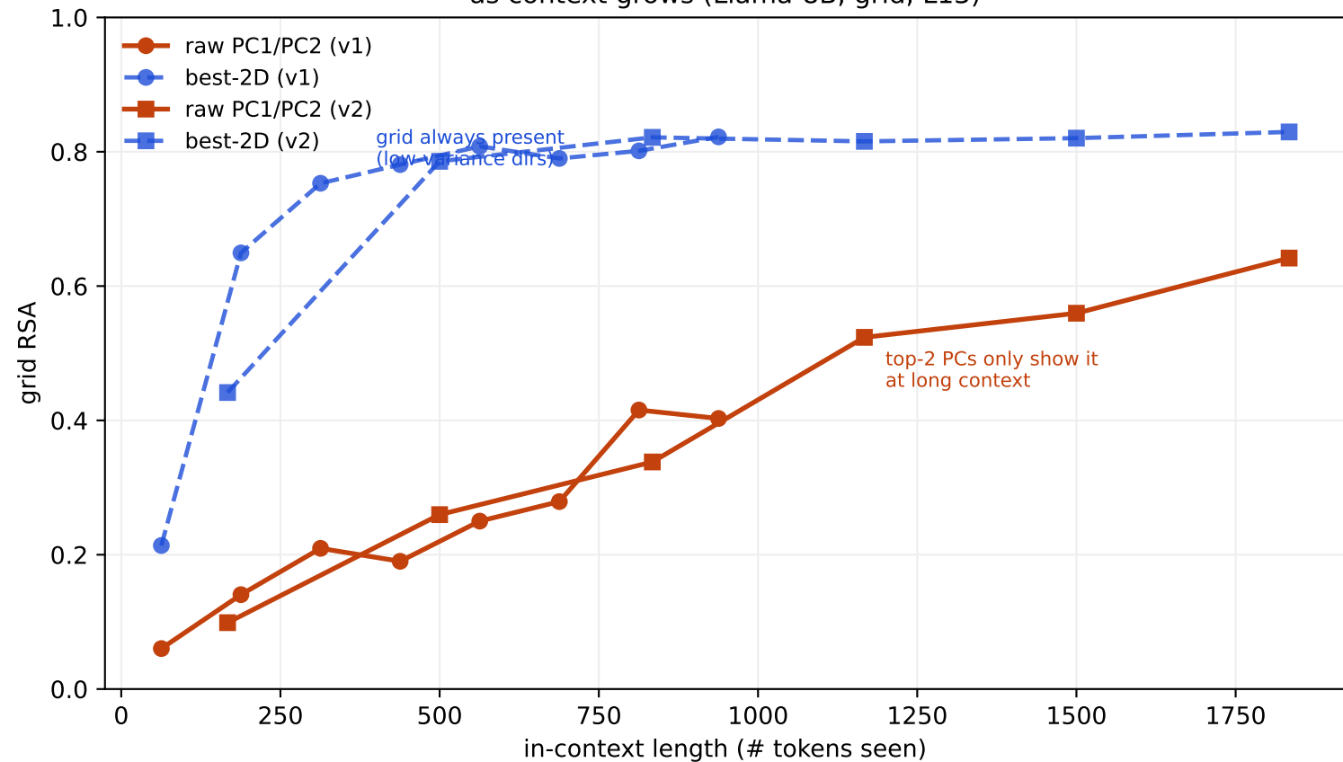
Why the raw PCA looked "messed up": the grid moves INTO the top-2 PCs as context grows (Llama-8B, grid, L13)
