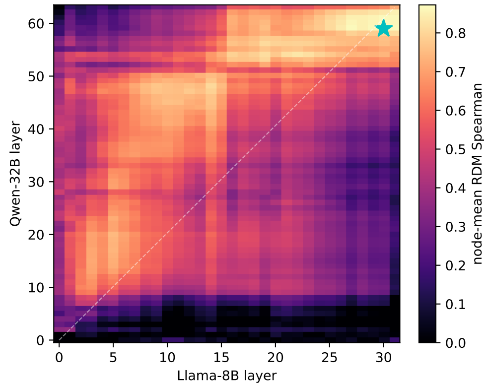
Qwen-32B vs Llama-8B (max RSA 0.87 @ L59/L30)
