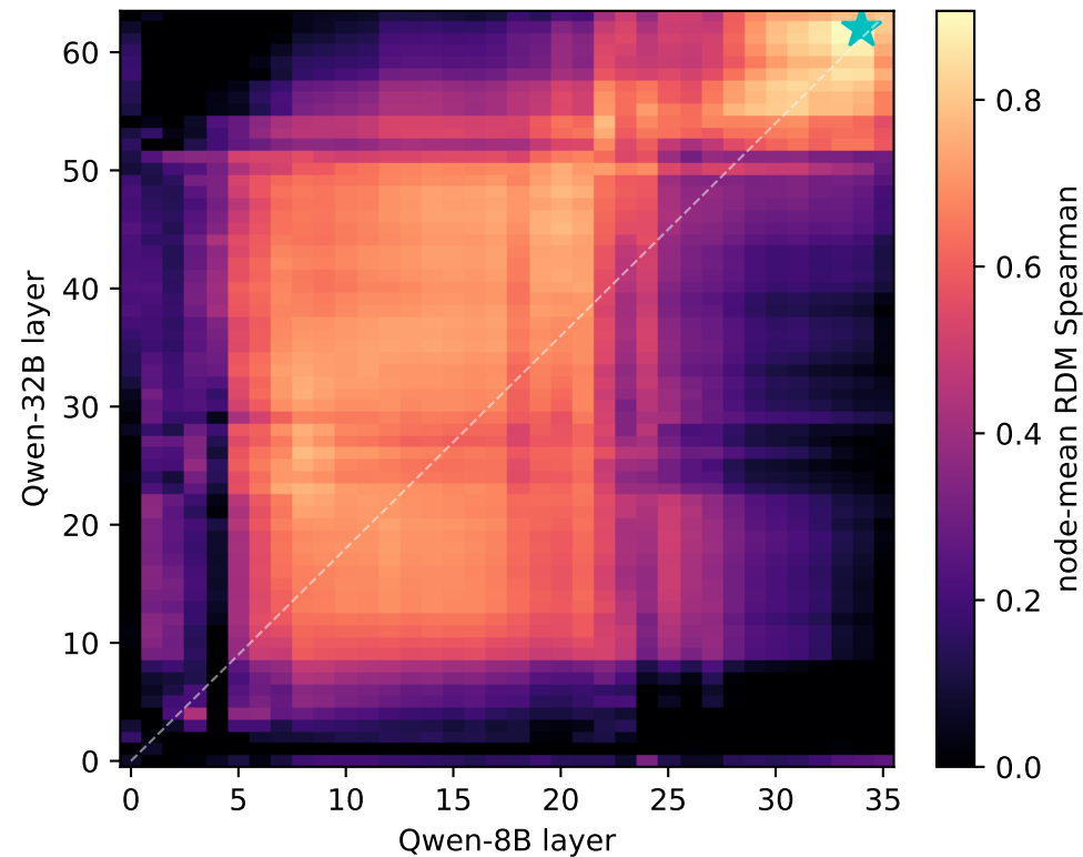
Qwen-32B vs Qwen-8B (max RSA 0.91 @ L62/L34)
