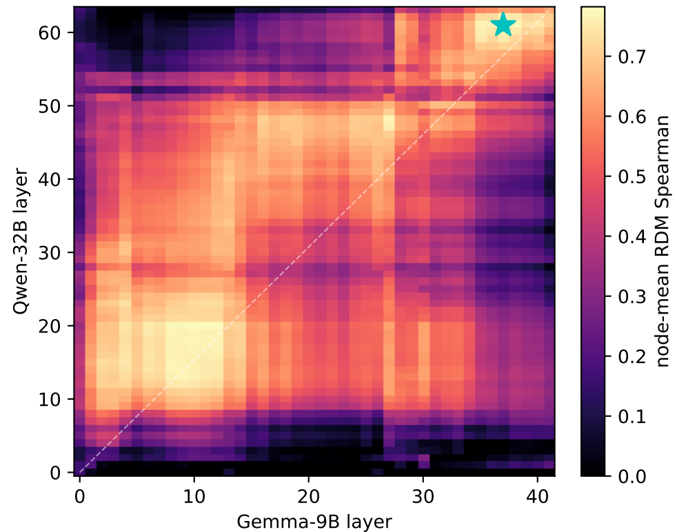
Qwen-32B vs Gemma-9B (max RSA 0.78 @ L61/L37)
