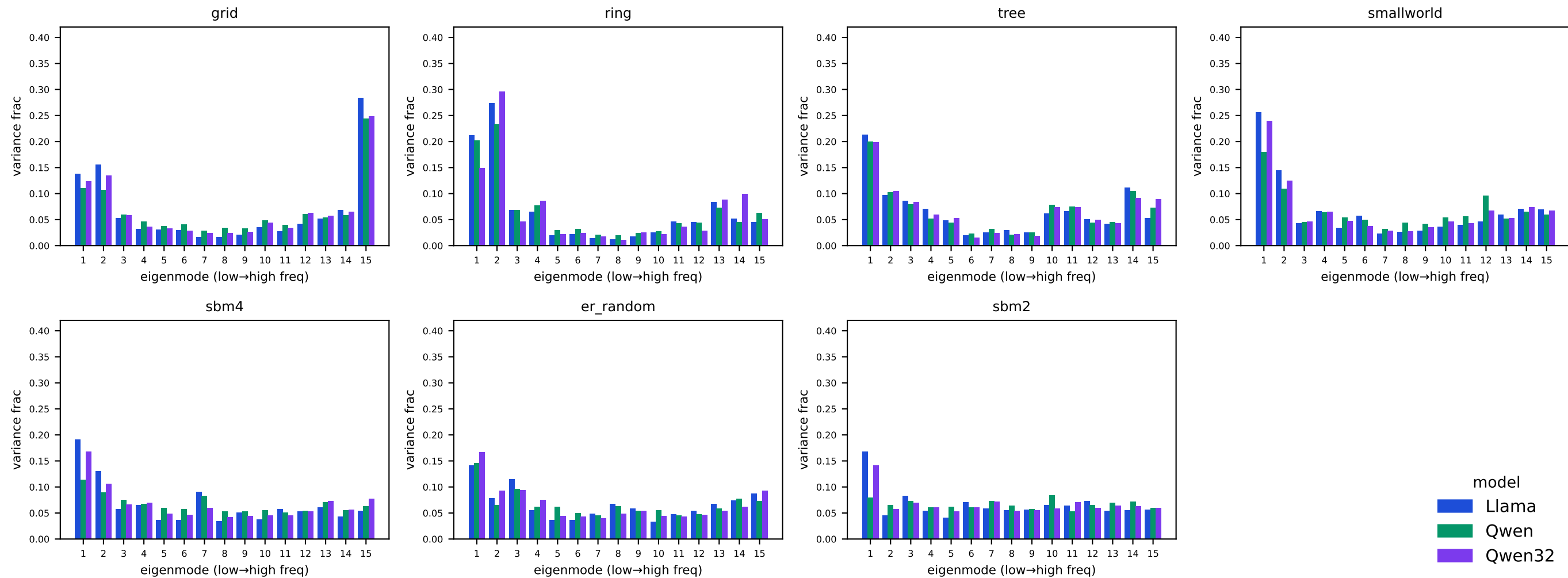
Node-mean variance vs Laplacian eigenmode, per family — Llama / Qwen / Qwen32
