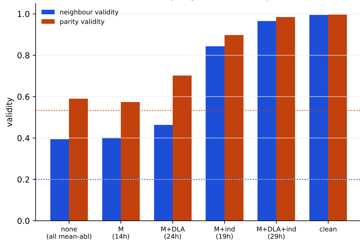
Mean-ablation keep-only circuits (MLPs kept clean)
