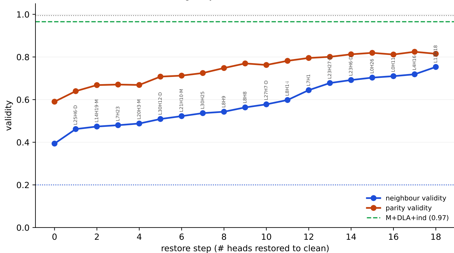
Additive greedy restore from all-mean-ablated
