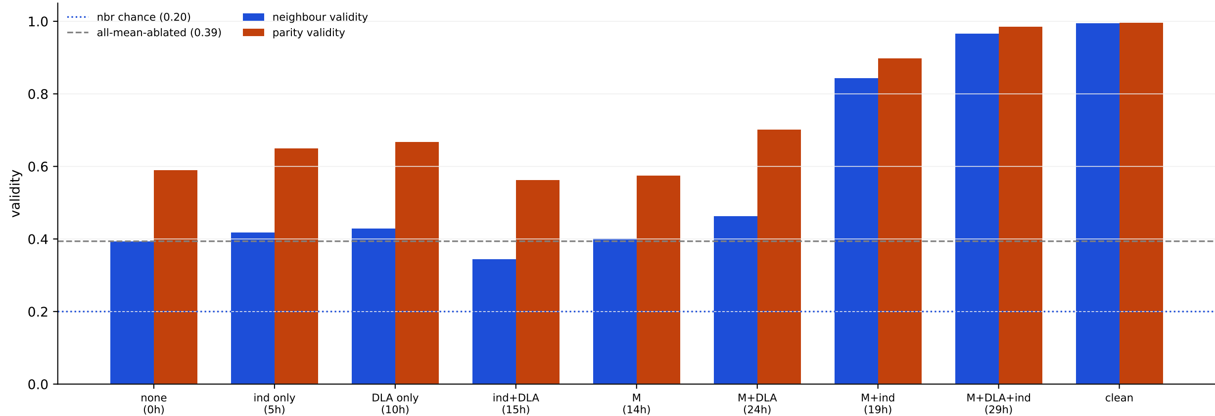
Minimum viable circuit (Llama, grid): builders (M) + movers (induction) are SYNERGISTIC no single block works alone; M+induction jumps to 0.84, +DLA readers → 0.97
