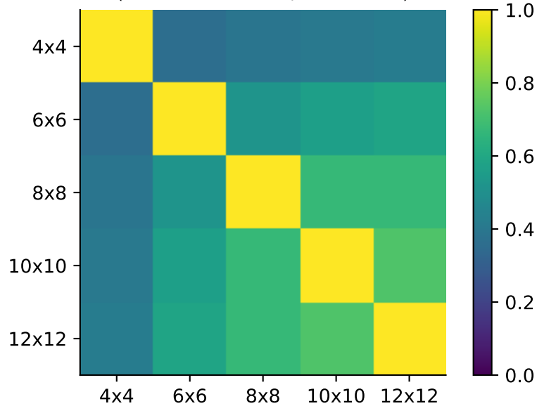
mean \cos^2 overlap of rank-16 DAS subspaces (random baseline 16/128 = 0.125 )
