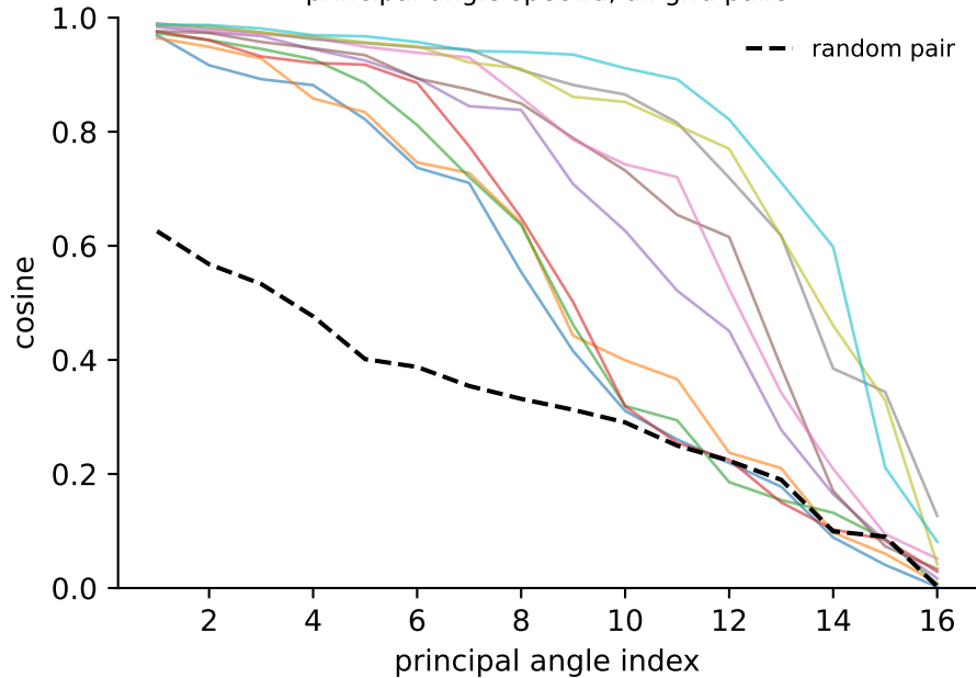
principal-angle spectra, all grid pairs
