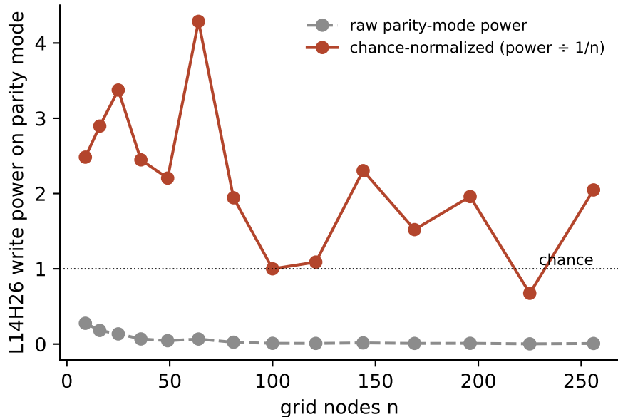
parity write enrichment persists to 16×16 (ctx 2000)
