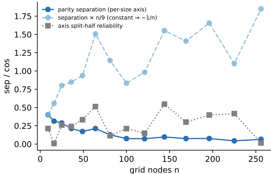
sep declines \sim 1/n = per-node sample statistics (converged: ctx 1000 \approx ctx 2000)
