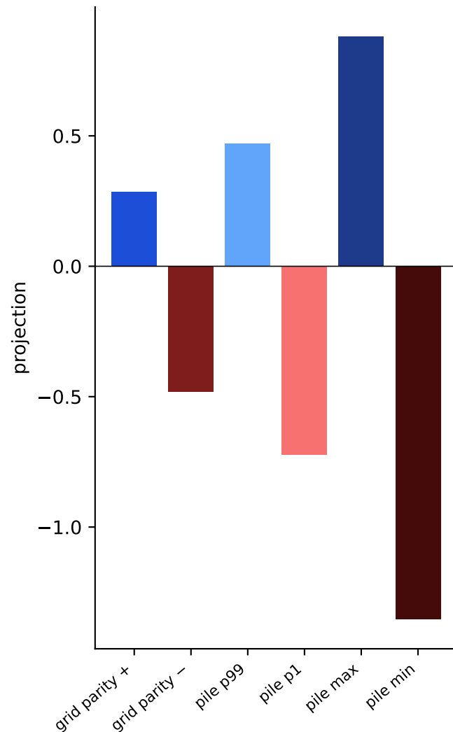
(b) Natural text fires the axis at GRID SCALE (pile max 0.88 ≈ grid +/− separation 0.77)
