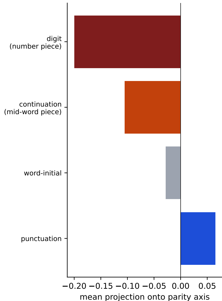
(a) The parity axis tracks token BOUNDARY: inside-unit (−) vs punctuation boundary (+)
