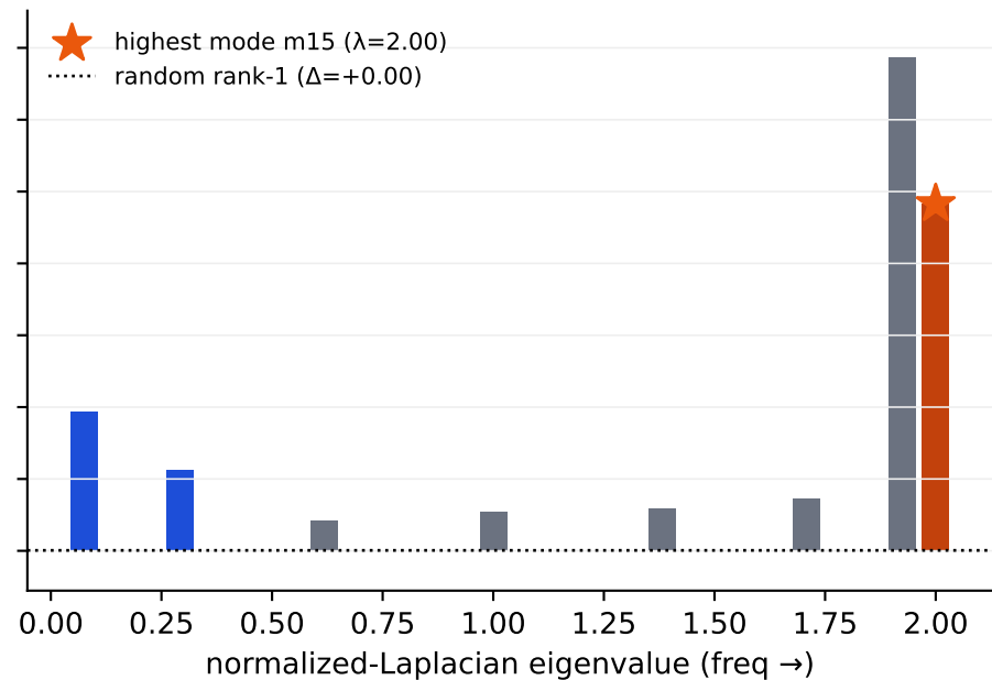
ring \lambda_{\max}=2.00 bipartite \rightarrow parity parity-validity=0.99
