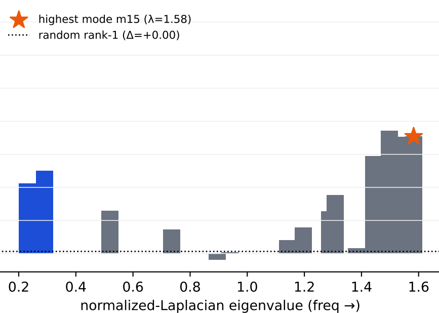
hex \lambda_{\max}=1.58 frustrated: no parity parity-validity=0.65
