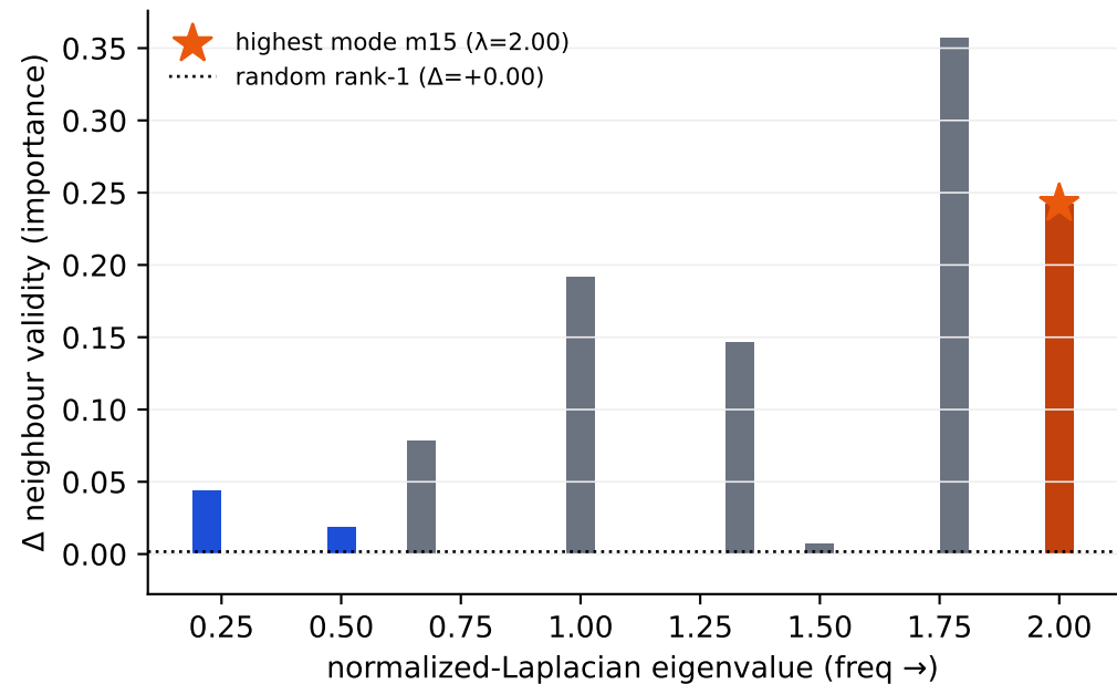
grid \lambda_{\max}=2.00 bipartite \rightarrow parity parity-validity=1.00
