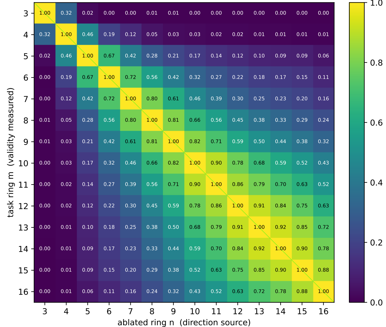
REPRESENTATIONAL alignment — direction-subspace similarity (mean \cos^2 principal angles, layer 30)
