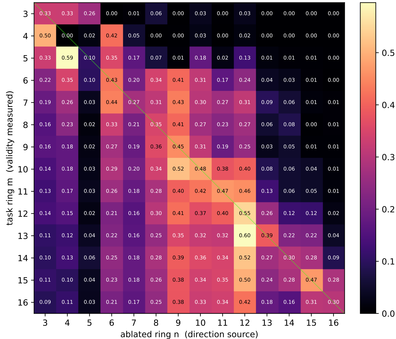
CAUSAL circuit sharing — fractional drop in ring-m validity when ablating ring-n's fundamental direction
