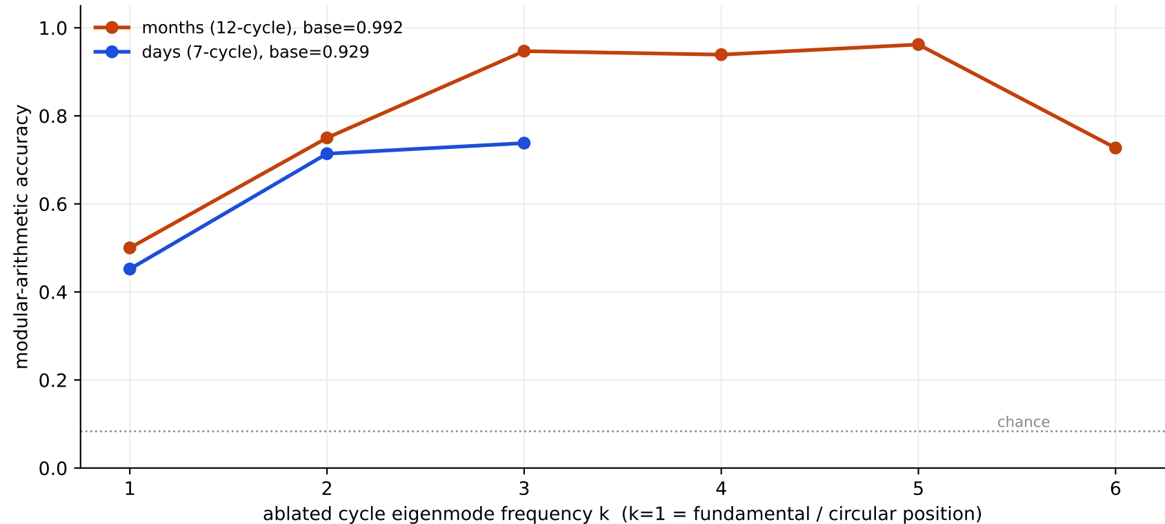
Ablating each eigenmode of the 12-cycle (months) / 7-cycle (days) the FUNDAMENTAL (k=1) is the causal circle
