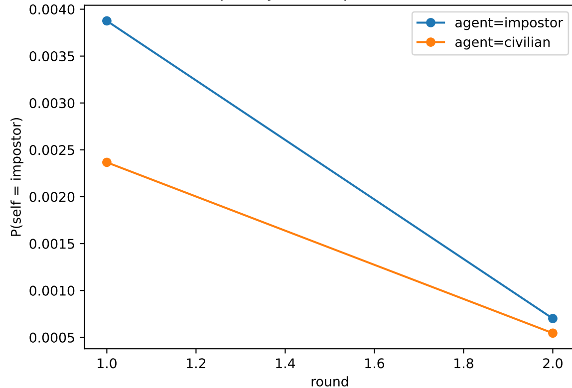
belief trajectory (forked per-round elicitation)
